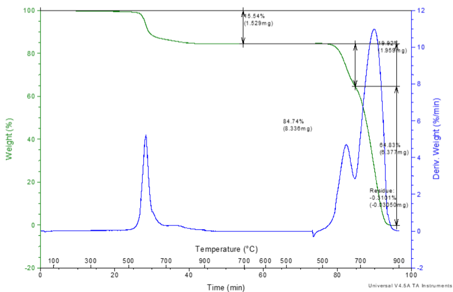
(b) TGA plot of scrap tape sample.
