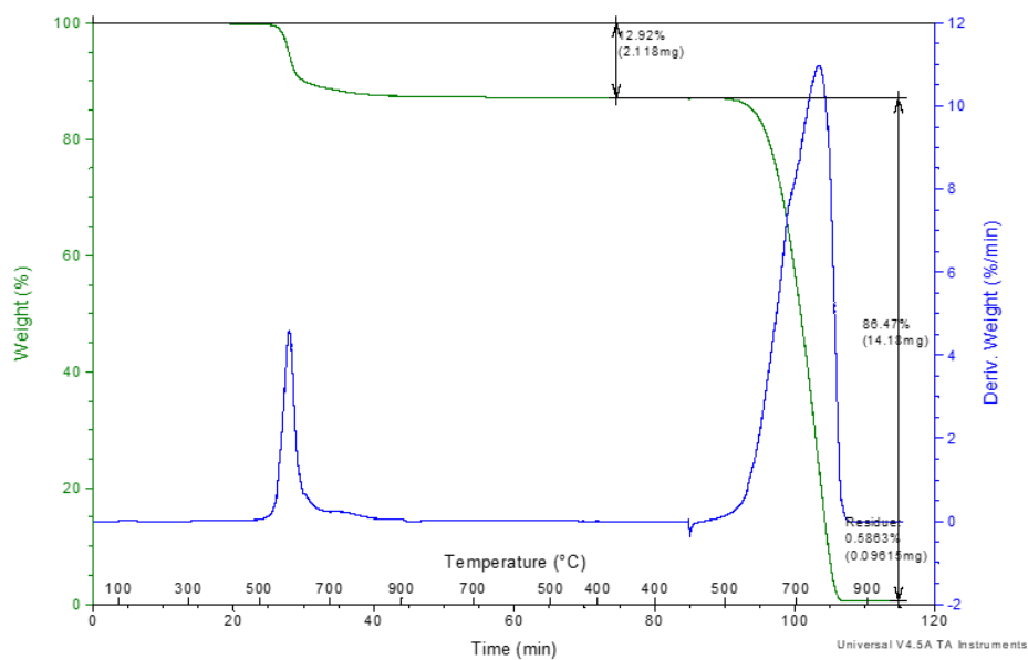
(a) TGA plot of the virgin PEKK/AS4 sheet.
