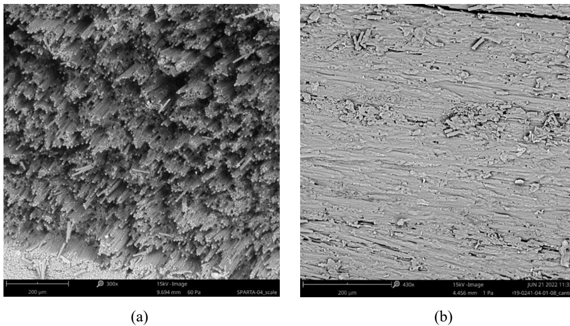
Figure S2. The SEM images show the cross section of the virgin [0]_{16} panel (a) and the recycled composite panel (b) (scale 200 \mu\text{m} ).
