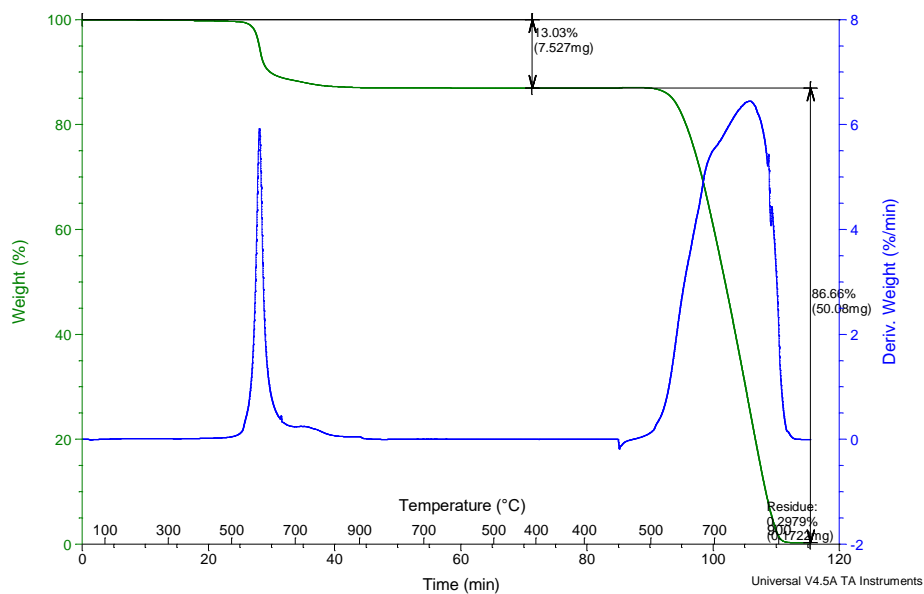
(a) TGA plot of the virgin panel.
