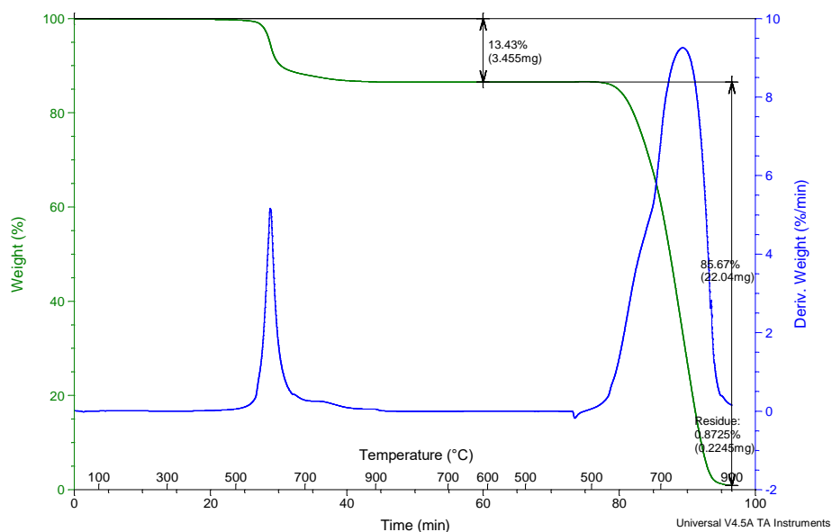
(b) TGA plot of recycled panel.
