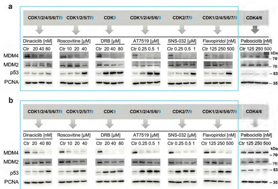
Fig. 2 Pan-CDK inhibitors predominantly target MDM4 expression in melanoma and breast carcinoma cells. Palbociclib, lacking activity toward CDK9, affects neither MDM4 nor MDM2 levels. Western blot analysis of cancer cell lysates after 24-h treatment with the indicated concentrations of CDK inhibitors in A375 (a) and MCF7 cells (b).
