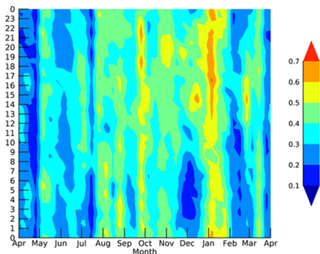
Fig. 4. Probability of the surface wind speed being 3 \text{ ms}^{-1} or less as a function of month and local time at Syowa Station during April 2016 to March 2019.
