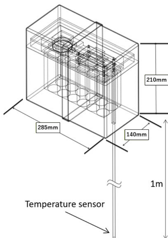
Fig. 3. Overview of balloon-borne instrument. Cylinders inside are batteries. The housing consists of an upper lid and a lower body.
