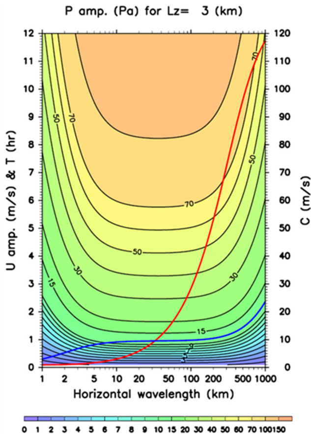
Fig. 1. Pressure amplitude (Pa) of gravity wave as a function of horizontal wavelength and horizontal wind amplitude, assuming a vertical wavelength of 3 km and a pressure level of around 60 hPa. Red and blue lines represent intrinsic period (hr) and intrinsic phase velocity ( \text{ms}^{-1} ) of gravity wave, respectively.
