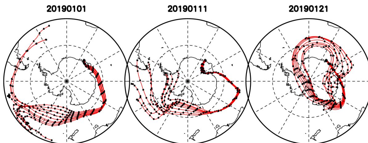
Fig. 5. 30day forward trajectories on a constant density surface starting at 65 hPa from Syowa Station. Initial 9 air parcels are put at (39.6E \pm 1.0 \text{ deg}, 69.0S \pm 0.5 \text{ deg}) on 1, 11, and 21 Jan. 2019. Dots are plotted every 1 day.
