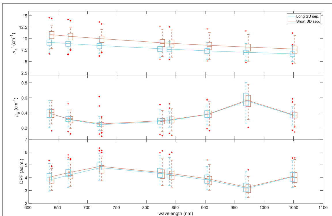
Figure 3. (Upper panel) The measured reduced scattering coefficient, (center panel) the absorption coefficient, and, (lower panel) differential pathlength factor of the sternocleidomastoid muscle over different wavelengths at both long and short SDSs is shown. The average over all subjects (solid lines) is shown together with a boxplot. Outliers are marked in red.
