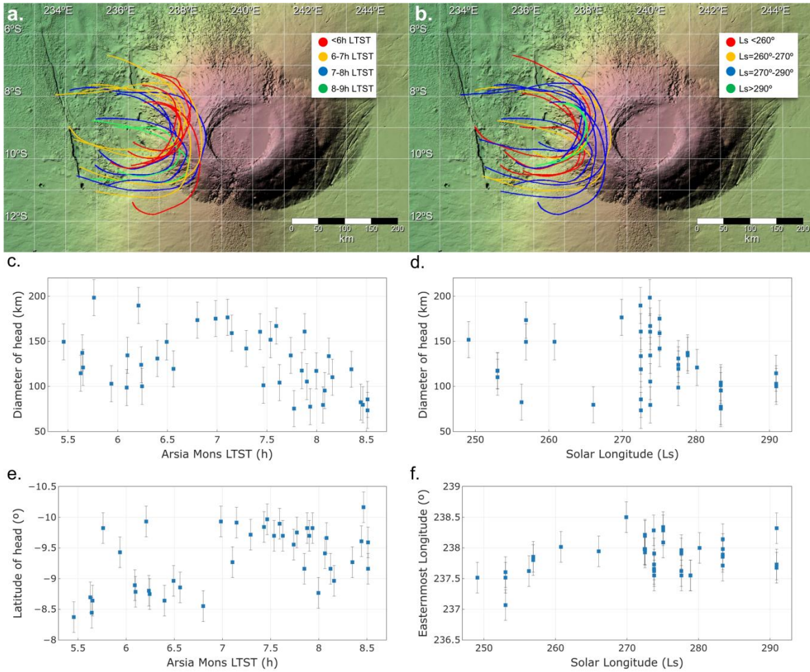
Figure 8. Panels a and b: Position and size of the head of the AMEC as a function of LTST and Solar Longitude. The curves (traced manually) represent the head contour and colors identify LTST in (a) and Ls in (b). Panels (c) and (d) Head diameter as a function of LTST and Ls. (e) Latitude of the head center as a function of LTST. (f) Longitude of the head center as a function of Ls.
