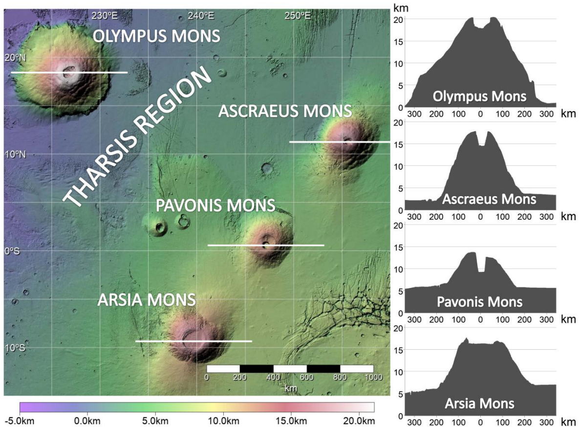
Figure 4. Topography of the Tharsis region from MOLA-HSRC data plot with hillshading (Ferguson et al., 2018). The four giant volcanoes are apparent. Right panels show topographic profiles for each volcano from MOLA. Altitudes are relative to the areoid.
