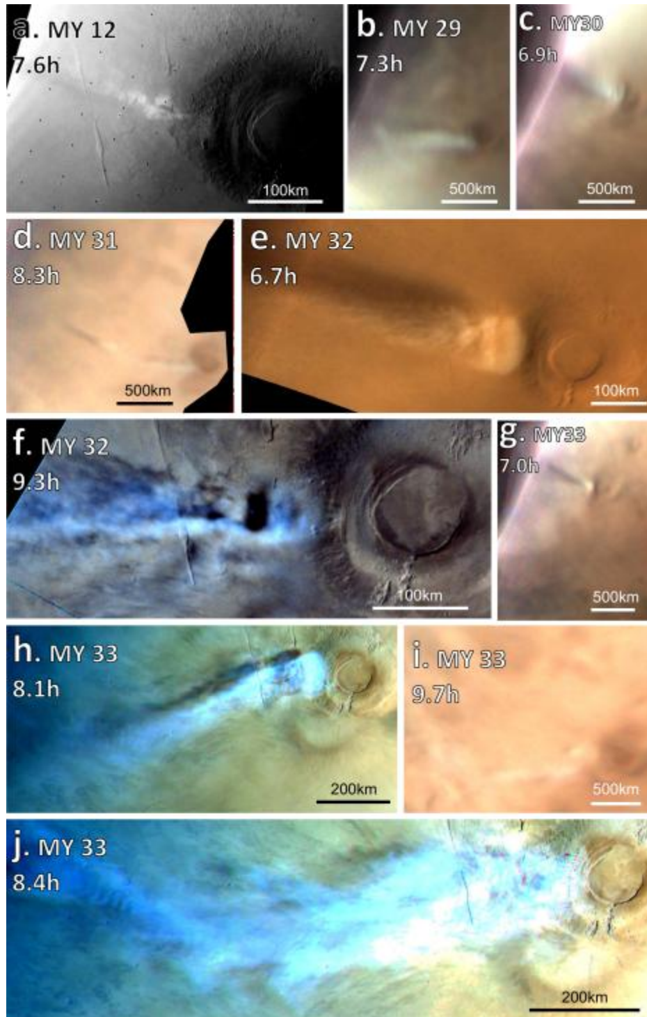
Figure 11. Images of the AMEC phenomenon seen in different MYs. All images are projected onto cylindrical maps. Spatial scale is indicated in each panel. (a) MY 12. 1977-08-11, Ls 314° (Viking Orbiter 2 observation 356b33). (b) MY 29. 2009-07-2, Ls 296° (VMC observation 090025). (c) MY 30. 2011-03-21, Ls 258° (VMC observation 110005). (d) MY 31. 2012-12-15, Ls 226° (VMC observation 120060). (e) MY 32. 2014-12-13, Ls 252° (MCC product MCC_MRD_20141213T134802312_D_GDS). (f) MY 32. 2015-01-04, Ls 266° (MCC product
