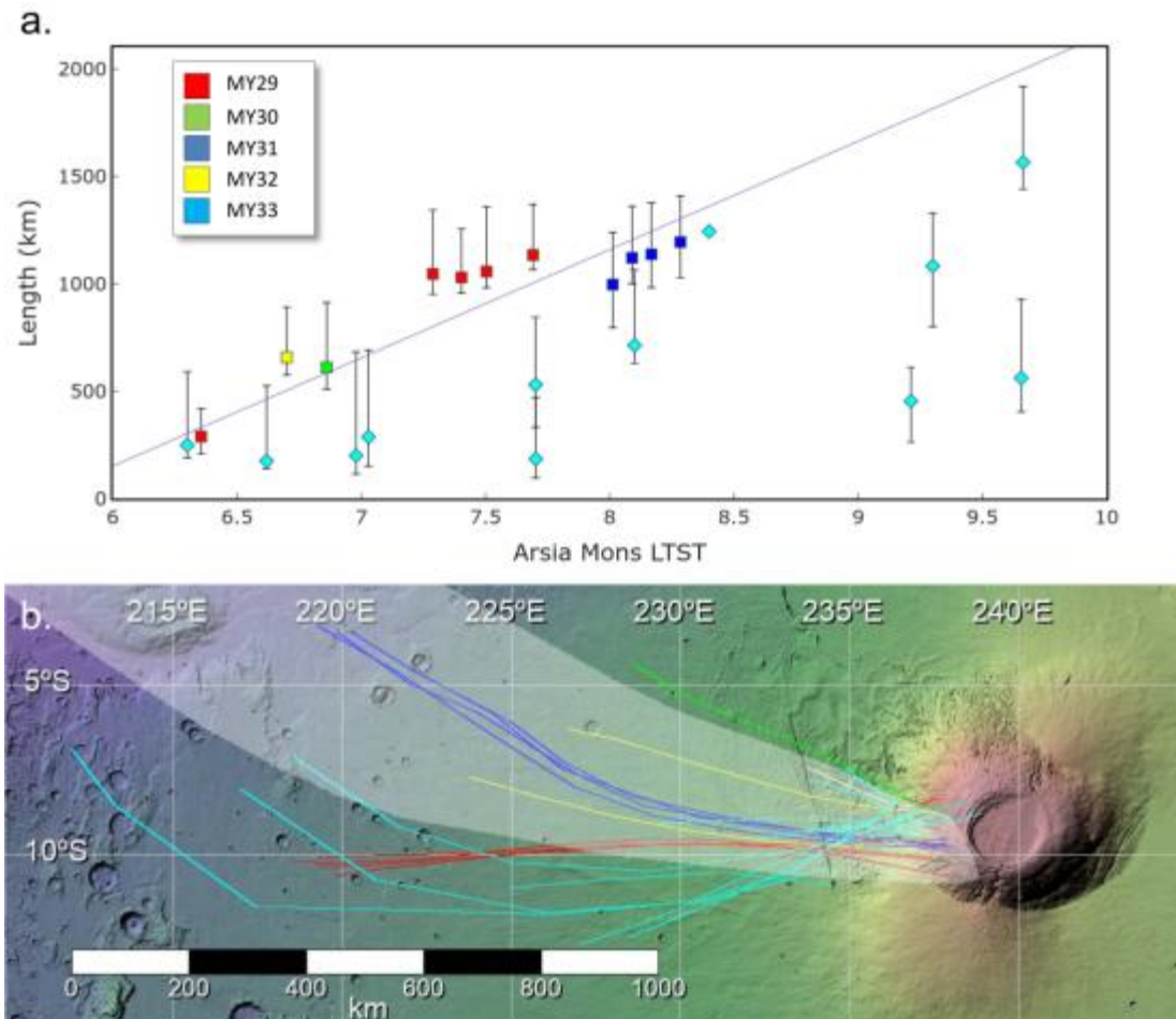
Figure 12. Length and Curvature of the AMEC in MYs 29-33 (Analogous to Figure 6). Panel a. Length of the AMEC as a function of local time. Color code indicates MY. The linear fit corresponds to all data except for MY 33 (indicated with diamond shaped markers). Panel b. Outline of the tail of the cloud over a topographic map as in Figure 6b. The area occupied by the cloud trajectories in MY 34 (Fig. 6b) is indicated by a background white shadow for comparison.
