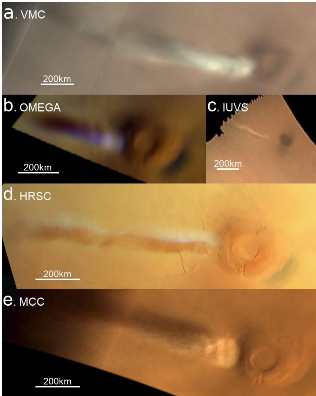
Figure 3. Examples of images from different instruments. Panels a to e show cylindrical projections of images displaying the AMEC at Arsia Mons. (a) VMC observation. 2018-10-22, MY 34, Ls 274°, LTST 7.8. (VMC observation 180371). (b) OMEGA observation. 2018-09-17, MY 34, Ls 252°, LTST 7.5. (MEX orbit 18612). (c) IUVS observation from apocenter. 2018-09-07, MY 34, Ls 245°, LTST 8.9. (MAVEN orbit 7673). (d) HRSC observation. 2018-09-21, MY 34, Ls 254°, LTST 8.5. (MEX orbit 18627). (e) MCC observation. 2014-12-13, MY 32, Ls 252°, LTST 6.7. (MCC product MCC_MRD_20141213T134802312_D_GDS).
