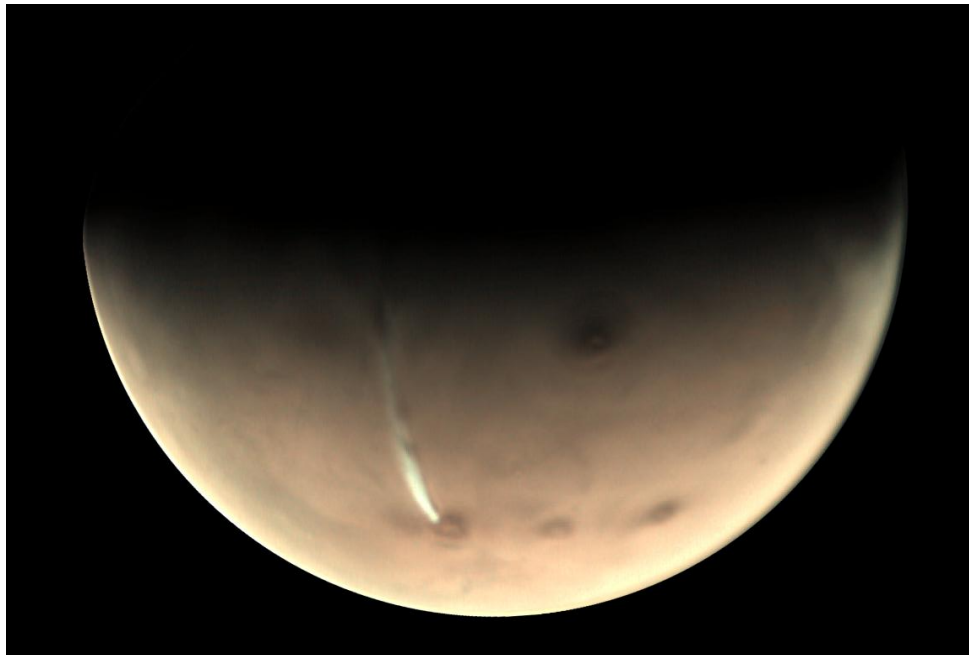
Figure 1. The elongated cloud extending around 1800 km to the west from Arsia Mons volcano on October 10 2018 (MY34). Image acquired by the VMC camera on board MEX. ESA press release:
