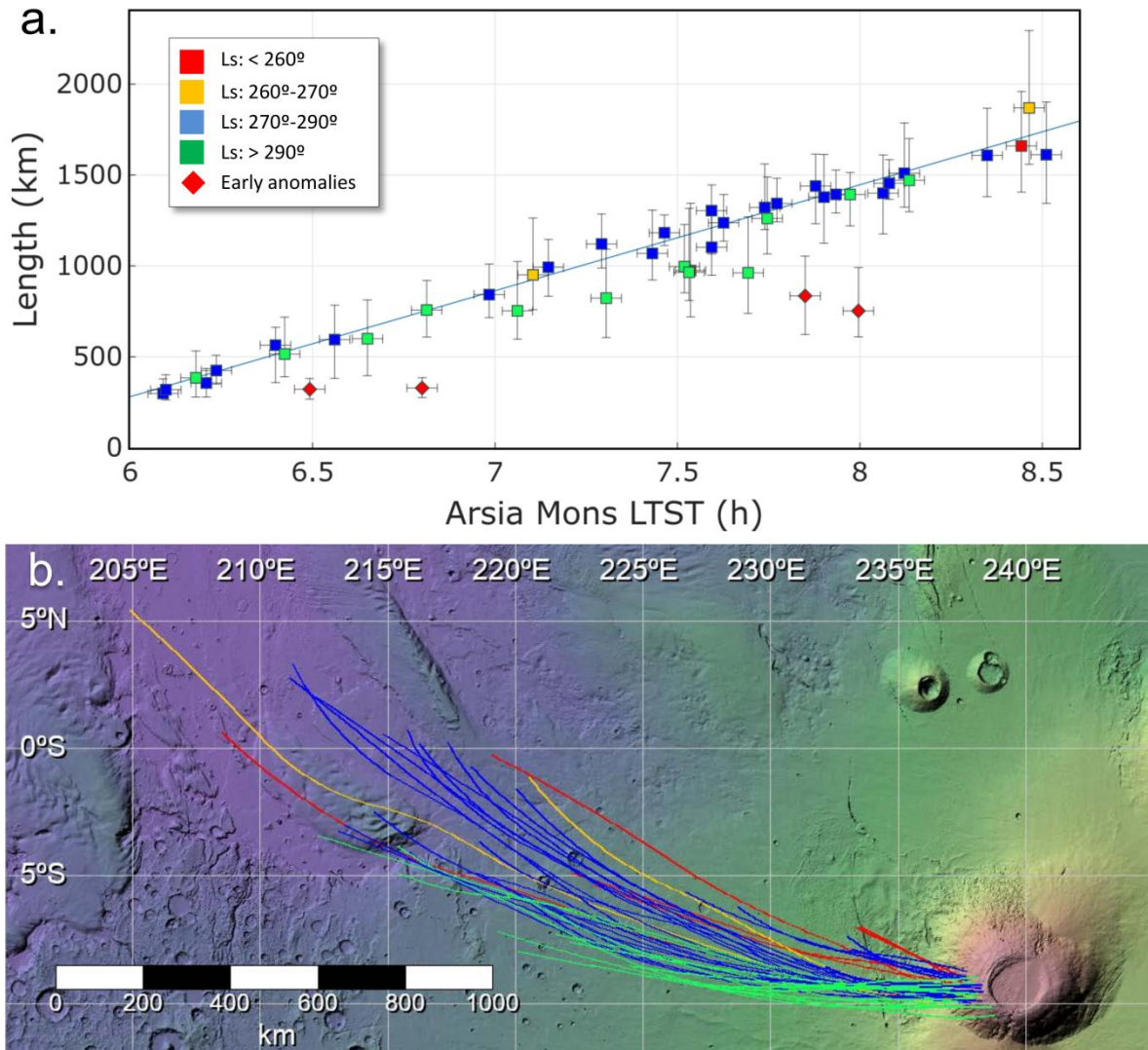
Figure 6. Expansion phase of the AMEC. (a) Length of the cloud as a function of LTST. Point incertainties are calculated as explained in Supplementary Text S3 . For long observations, only a representative part of all the available images are represented, separated by \sim 15 min. Linear fit (early anomalies excluded) gives an expansion velocity of 170 \pm 10 \text{ ms}^{-1} ; (b) Cloud trajectories (traced manually) on a topographic map, the same map as seen in Fig. 4. Color codes indicate the Ls ranges given in the legend in panel (a).
