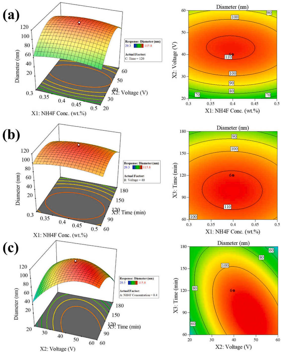
Fig. 4. 3D surface plot and its corresponding contour plot displaying the interactions between the variables affecting the diameter of the nanotubes: (a) \text{NH}_4\text{F} concentration and anodization voltage (keeping anodization time constant), (b) \text{NH}_4\text{F} concentration and anodization time (keeping anodization voltage constant), and (c) anodization voltage and time (keeping \text{NH}_4\text{F} concentration constant).
