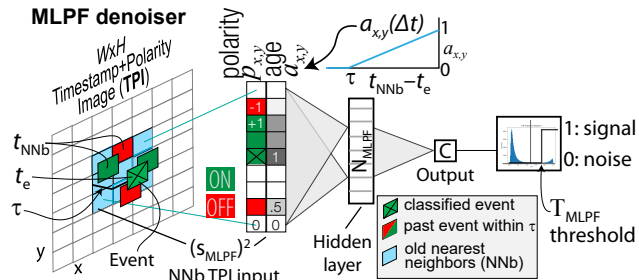
Figure 3. MLPF input and network.
