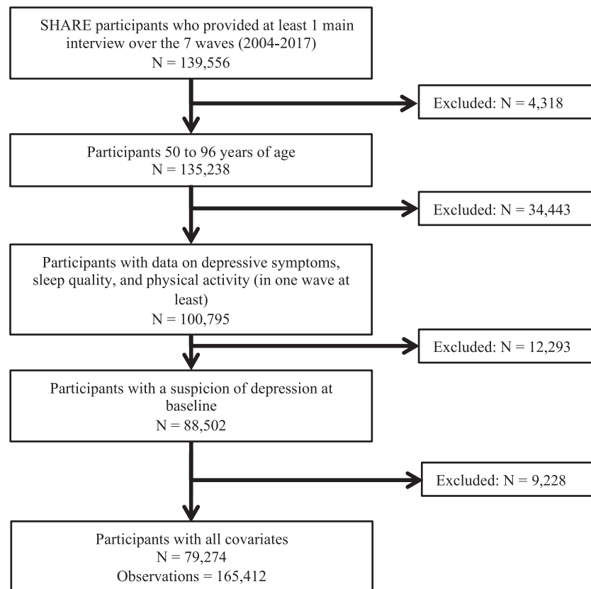
Fig. 1. Flowchart.
