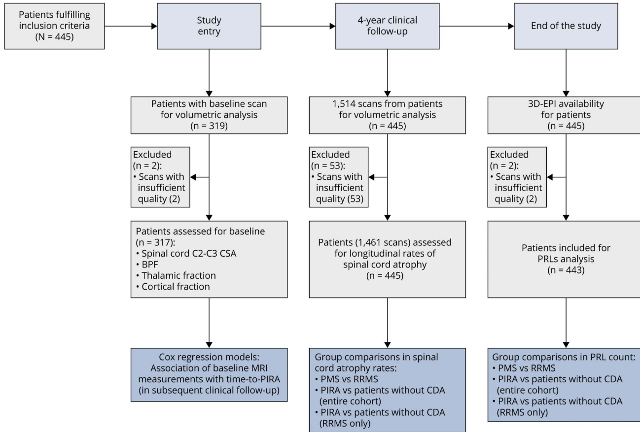
Figure 1 Study Design
