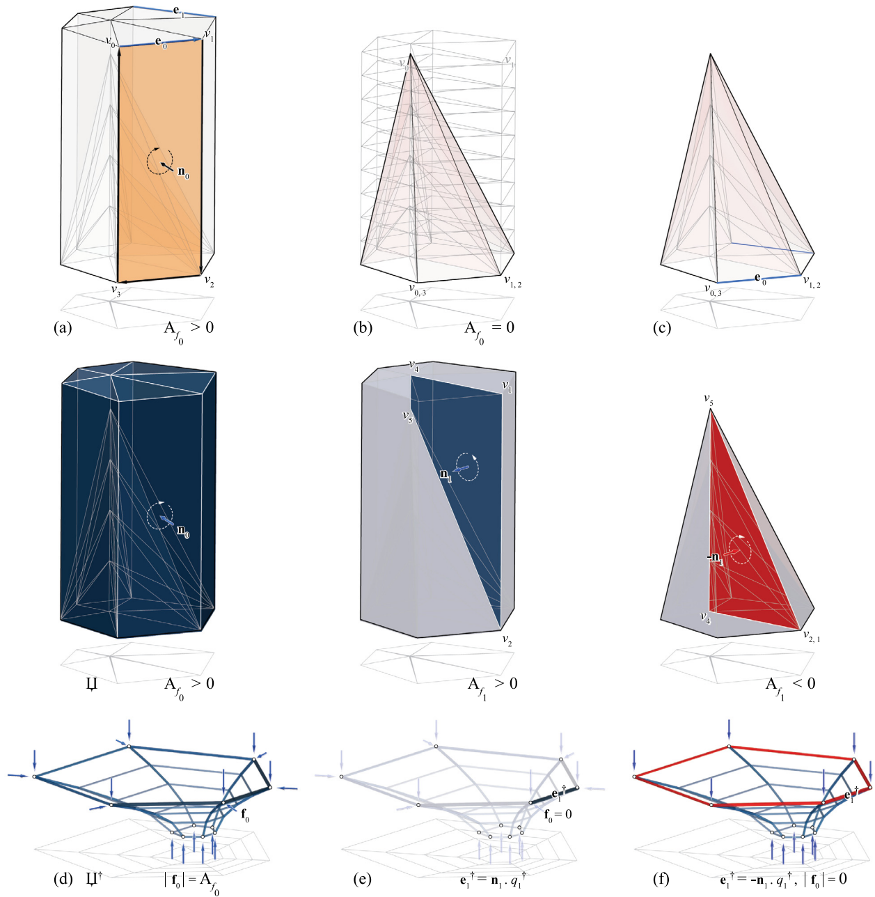
Fig. 15. (a) A force polyhedron and a selected face with zero area target, and two fixed edges on the top; (b) the transformation animation (for visualization purposes only); (c) the resulting force polyhedron where the selected face and all other side faces collapse to a line; (d), (e), and (f) the force and form diagrams and their transformation after changing the areas.
