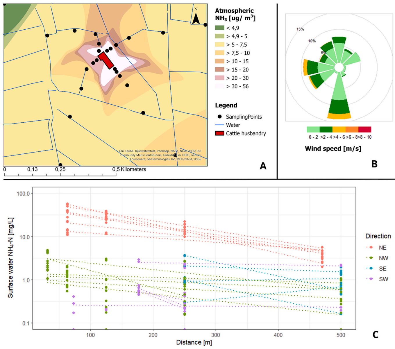
Fig. 2. Atmospheric \text{NH}_3 concentrations (A), wind rose (B) and surface water \text{NH}_4\text{-N} concentrations ( \text{mg}/\text{L} ) in relation to distance (m) to the stable (C) between 20 July 2021 and 13 October 2021. The atmospheric ammonia plot (A) was made by an Inverse Distance Weighing interpolation in ArcGIS pro 2.8. The wind rose shows where the wind originates from, and was constructed using data of the meteo station. The y-axis of plot (C) is displayed on a logarithmic scale. The different trendlines per wind direction indicate regression results from the six different time points (not coloured individually for visibility purposes). In (C): ‘NE’ = ‘Northeast’, ‘SE’ = ‘Southeast’, ‘SW’ = ‘Southwest’, ‘NW’ = ‘Northwest’.
