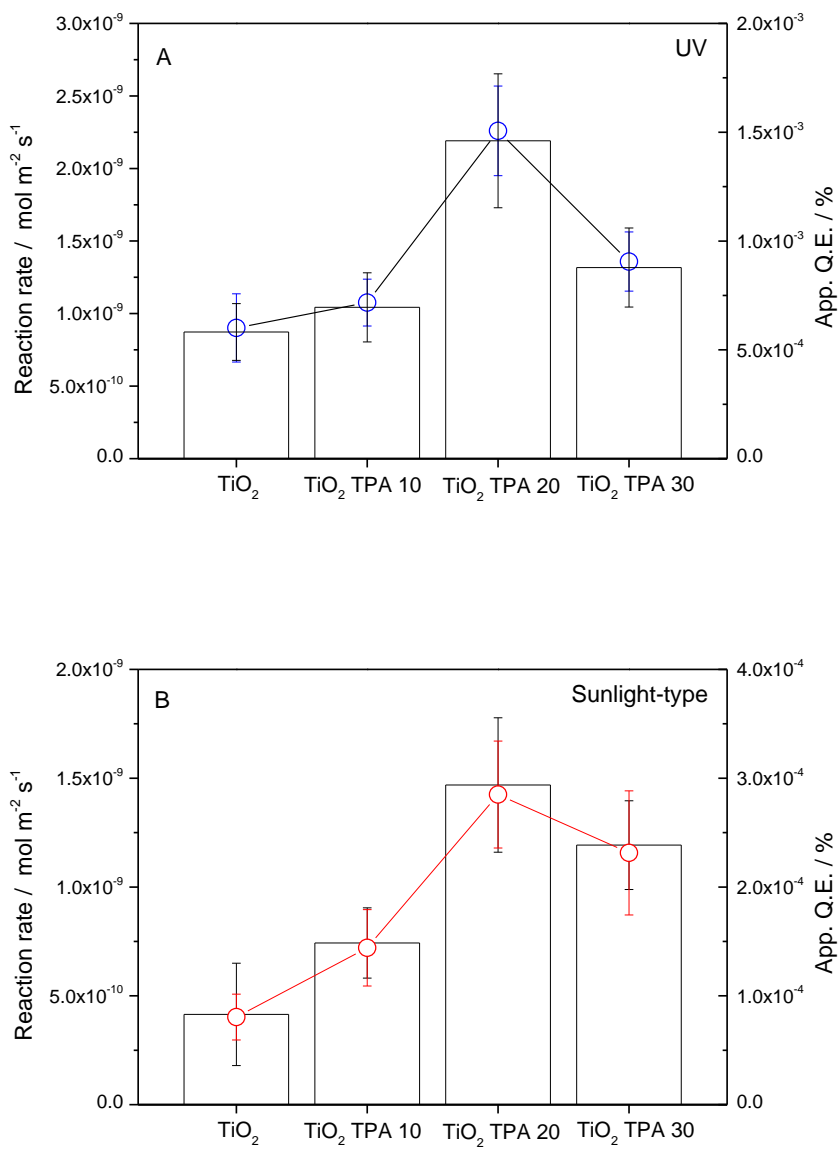
Figure 8. Reaction rate (columns) and apparent quantum efficiency (circles) under UV (A) and sunlight-type (B) irradiation conditions.
