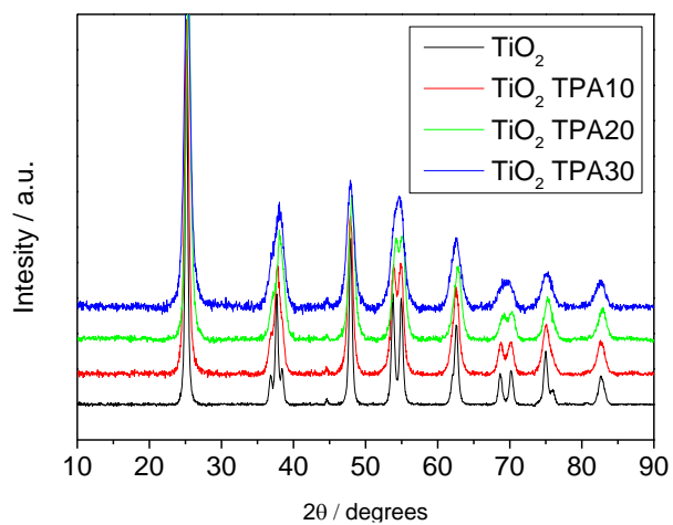
Figure 2. XRD patterns for the \text{TiO}_2 TPA (X) samples and Ti reference.
