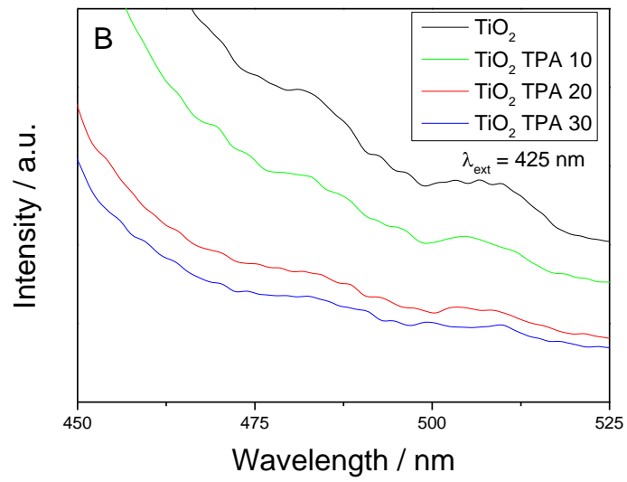
Figure 11. Photoluminescence spectra of the samples under UV (A) and Visible (B) excitation.
