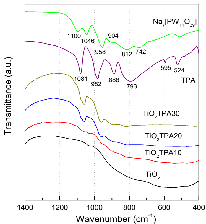
Figure 6. Infrared spectra of the composite and reference materials (bulk TPA and \text{Na}_7[\text{PW}_{11}\text{O}_{39}] ).
