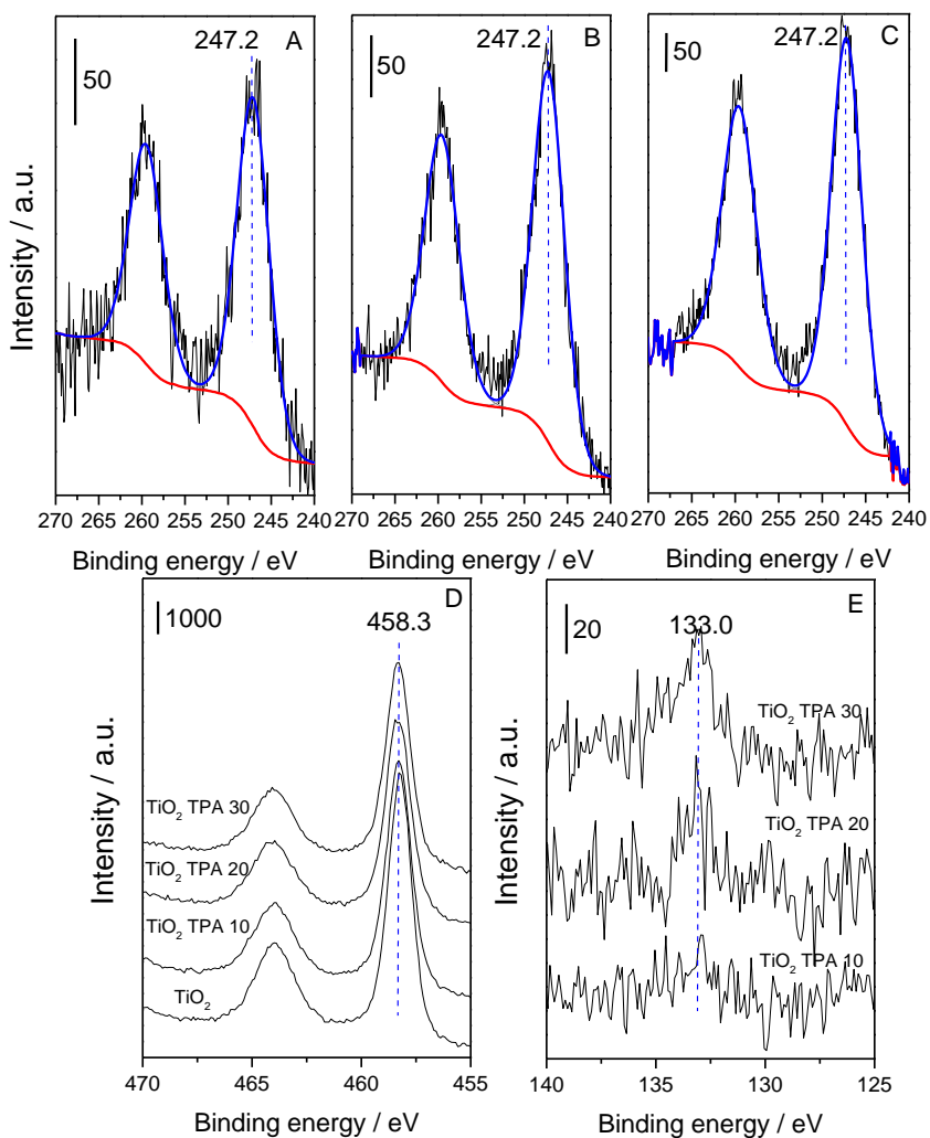
Figure 5. W 4d XPS spectra of the TiO 2 TPA10 (A), TiO 2 TPA20 (B) and TiO 2 TPA30 (C) sample, respectively. (D) Ti 2p XPS spectra of the TiO 2 TPA(X) samples and Ti references. (E) P 2p XPS spectra of the TiO 2 TPA(X) samples.
