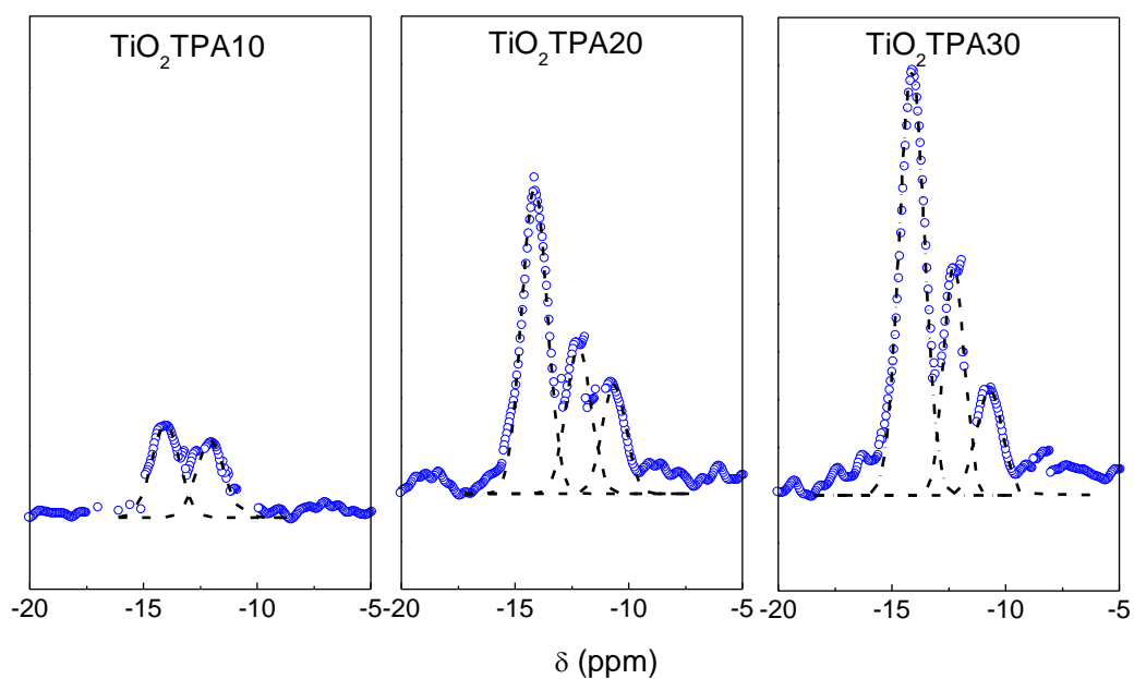
Figure 7. ^{31}\text{P} MAS-NMR spectra of the \text{TiO}_2 TPA(X) samples. Fitting results of the different P-containing species are presented.
