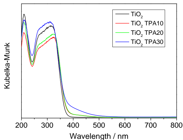
Figure 4. UV-vis for the TiO 2 TPA(X) samples and Ti reference.
