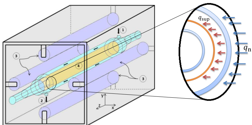
Figure 1. Photocatalytic annular reactor. (1) gas inlet, (2) gas outlet, (3) lamps, (4) catalyst sample.
