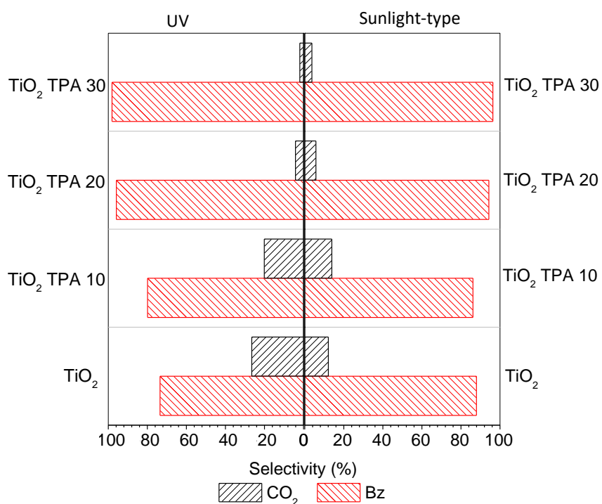
Figure 10. Selectivity to CO 2 and Benzaldehyde (Bz) for the Ti reference and TiO 2 TPA(X) samples.
