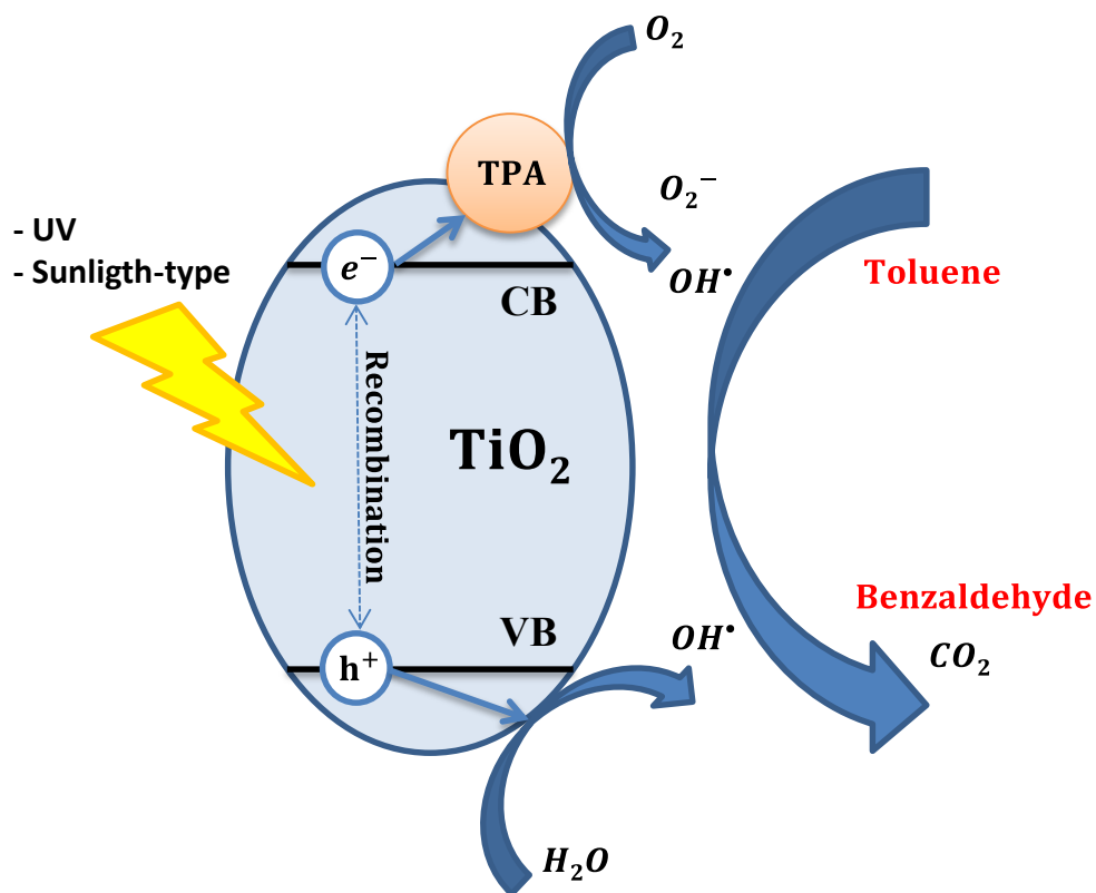
Scheme 1. Schematic representation of the main electronic events occurring after light irradiation (UV and Sunlight-type) and having an impact in the photodegradation of toluene.
