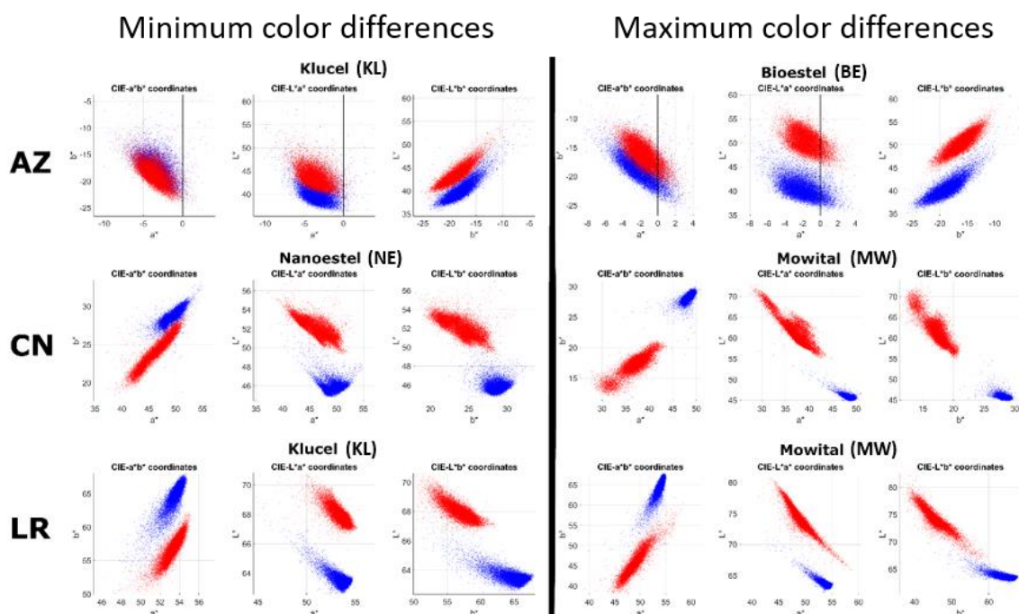
Figure 5: L^*a^*b^* plots for the minimum color difference (left three columns) and maximum color difference (right three columns). Data for AZ (first row), CN (second row) and LR (third row). Blue before the consolidant application and red: after. Please note the different scales used in some cases on the plots of the right and left groups.
