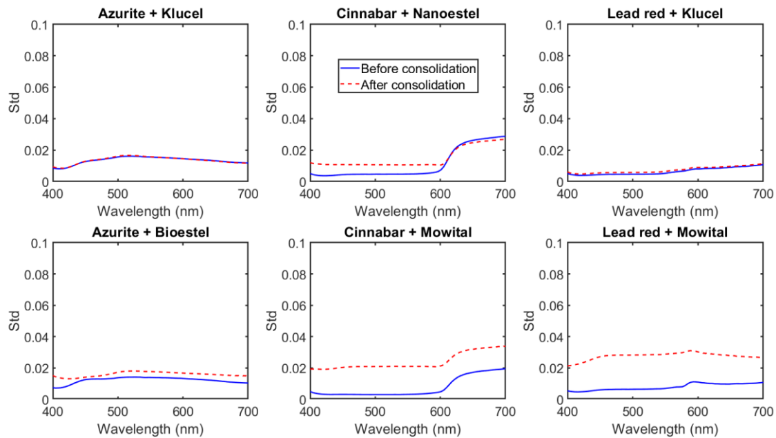
Figure 6: STD plots for the minimum color difference (upper row) and maximum color difference (lower row). Data for AZ (left column), CN (middle column) and LR (right column). Blue: before the consolidant application and red: after.
