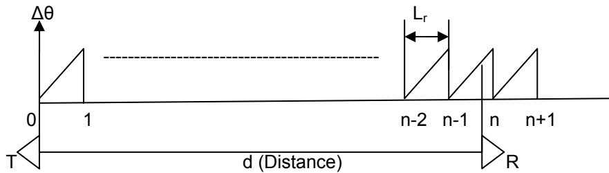
Fig. 3. Relation between d = c \cdot \Delta t and d = (n-1) \cdot L_r + (\Delta\theta/2\pi) \cdot L_r .
