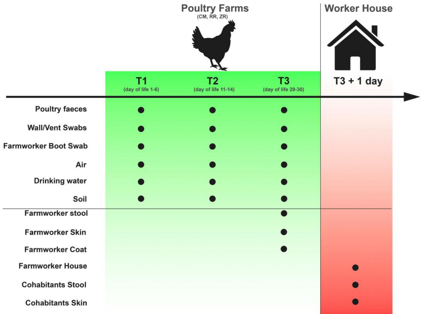
Fig. 1. Overview of the study design and sampling collection. Poultry and farm samples were collected at three different time points during the rearing cycle in three different Italian farms (CM, RR, ZR). Farm worker and cohabitant samples were taken at the last time point or the day immediately after. Black dots indicate the collection time points for each type of sample.
