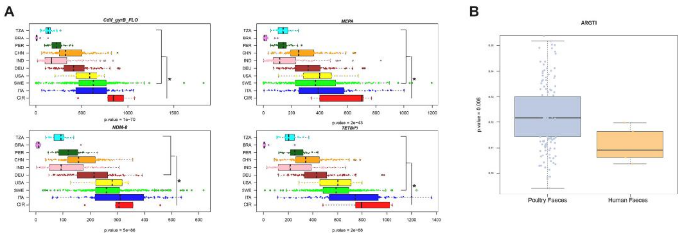
Fig. 8. Distribution of core mobile ARGs across different world populations. A) Boxplots showing reads per kilobase of genes per million reads mapped (RPKM) across 9 populations of the 4 most prevalent shared antibiotic resistance genes (ARGs) with prediction on plasmid or phage sequences, carried by the 180 shared species-level genome bins (SGBs) between poultry gut, internal farm, and human ecosystems. Human fecal samples from our study (CIR) showed a significant higher abundance of almost all genes compared to the other individuals (Wilcoxon rank sum test, p-value < 0.05). B) Boxplots showing the antibiotic resistance gene transferability index (ARGTI) values in poultry and human gut microbiomes (Kruskal-Wallis test, p-value < 0.001). TZA: Rural Tanzanian, BRA: Rural Brazilian, PER: Peruvian, CHN: Chinese, IND: Indian, DEU: German, USA: American, SWE: Swedish, ITA: Italian populations.
