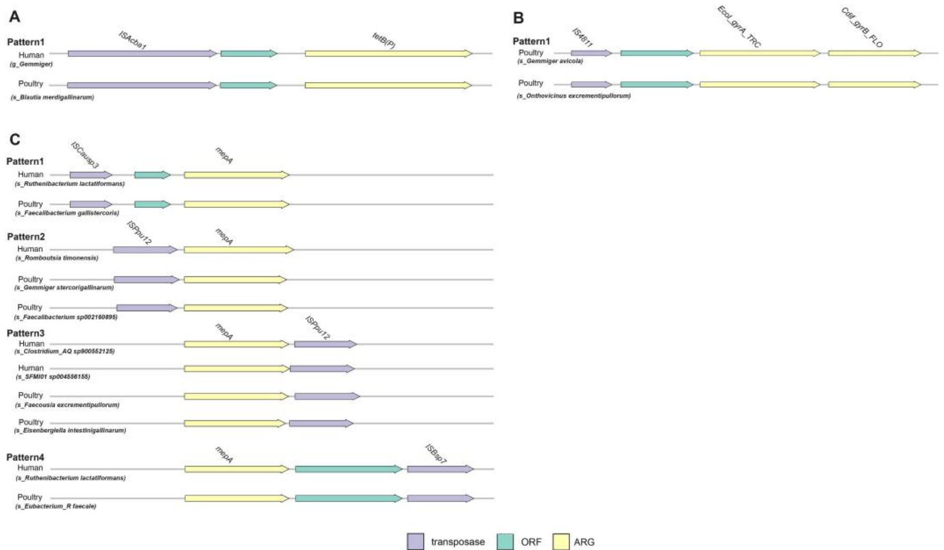
Fig. 7. Genomic structure patterns of antibiotic resistance genes across the shared species-level genome bins. Antibiotic resistance genes showing a prevalence higher than 75 % across the 180 species-level genome bins (SGBs) shared between poultry gut, internal farm, and human ecosystems with a prediction on plasmid or phage sequences highlight in some case the same genomic structure. Antibiotic resistance genes (ARGs) patterns for tetB(P) (A), Cdif_gyrB_FLO (B) and mepA (C) that were shared among different species-level genome bins (SGBs) with their identified lowest taxonomic level are highlighted under each genomic pattern. A color legend of the coding DNA sequences (CDSs) is located at the bottom of the figure, highlighting antibiotic resistance genes, transposases, and other open reading frames (ORFs).
