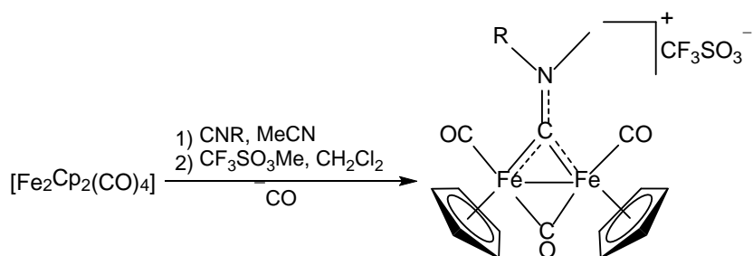
Scheme 1. Synthesis in two steps of diiron cationic \mu -aminocarbonyl complexes from [\text{Fe}_2\text{Cp}_2(\text{CO})_4] (R = alkyl, aryl).
