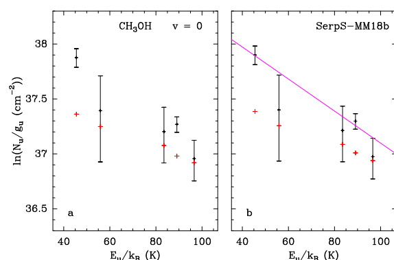
Fig. E.69. Same as Fig. E.1 but for CH 3 OH in SerpS-MM18b.
