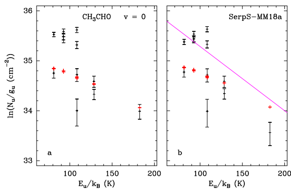
Fig. E.64. Same as Fig. E.1 but for CH 3 CHO in SerpS-MM18a.
