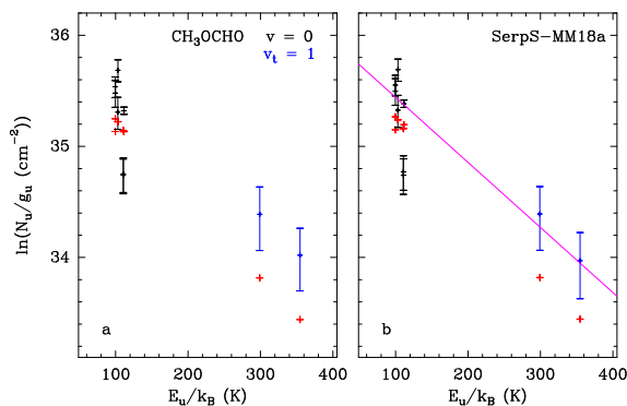
Fig. E.63. Same as Fig. E.1 but for CH 3 OCHO in SerpS-MM18a.
