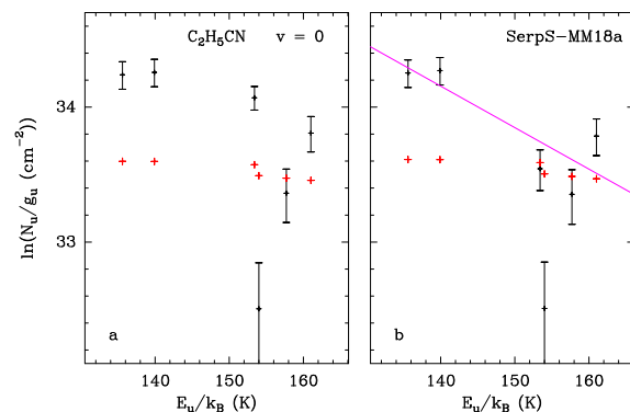
Fig. E.67. Same as Fig. E.1 but for C 2 H 5 CN in SerpS-MM18a.
