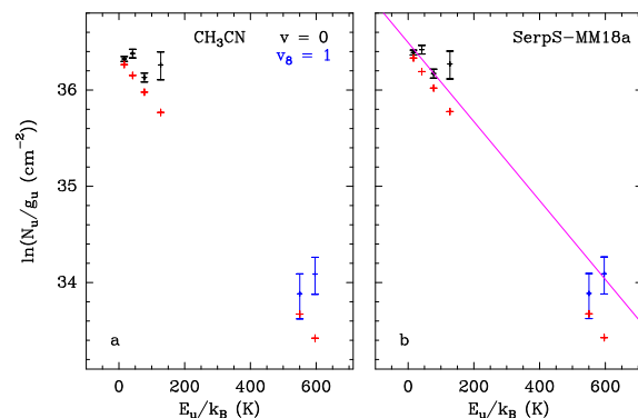
Fig. E.66. Same as Fig. E.1 but for CH 3 CN in SerpS-MM18a.
