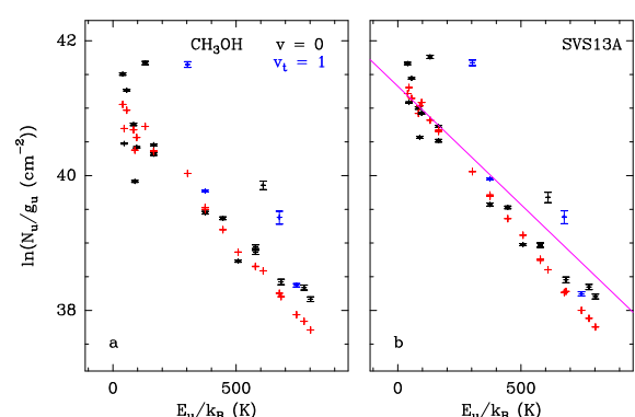
Fig. E.21. Same as Fig. E.1 but for \text{CH}_3\text{OH} in SVS13A.
