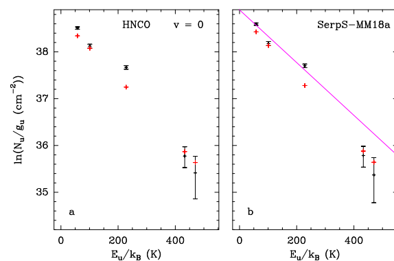
Fig. E.68. Same as Fig. E.1 but for HNCO in SerpS-MM18a.
