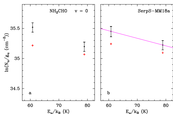
Fig. E.65. Same as Fig. E.1 but for NH 2 CHO in SerpS-MM18a.
