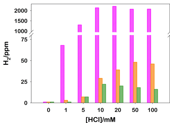
Figure 6. Photoproduced H_2 obtained upon 180 s irradiation at 460 nm of 2 mL [Ru(bpy)_3]^{2+} (25.0 \mu M ), MV^{2+} (5.0 mM), TPP (0.1 M), and RuO_2 (0.04 mg) in acetonitrile (pink), dimethylformamide (orange), and dimethyl sulfoxide (green) at different HCl concentrations in the Arduino sensor.
