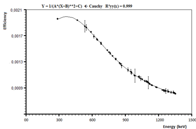
Figure 1. Efficiency curve with ^{166\text{m}}\text{Ho} , ^{152}\text{Eu} , ^{133}\text{Ba} , ^{137}\text{Cs} , ^{241}\text{Am} , ^{54}\text{Mn} and ^{65}\text{Zn} radionuclidic standards
