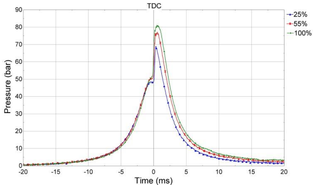
Figure 7. Cylinder pressure for the test with Diesel S10, CR = 20:1, SOI = 212.6 mm (1.43 ms before TDC) and 1750 rpm.
