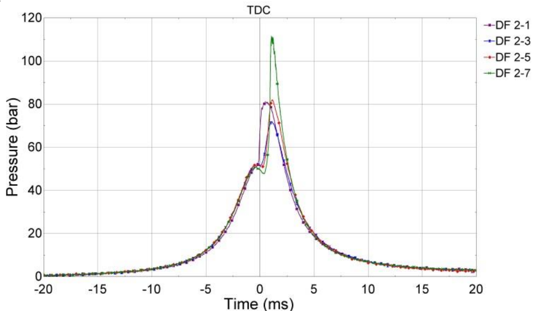
1. Figure 10. Cylinder pressure for the test with Diesel S10 and H100, CR = 20:1, 100% load and 1750 rpm.
