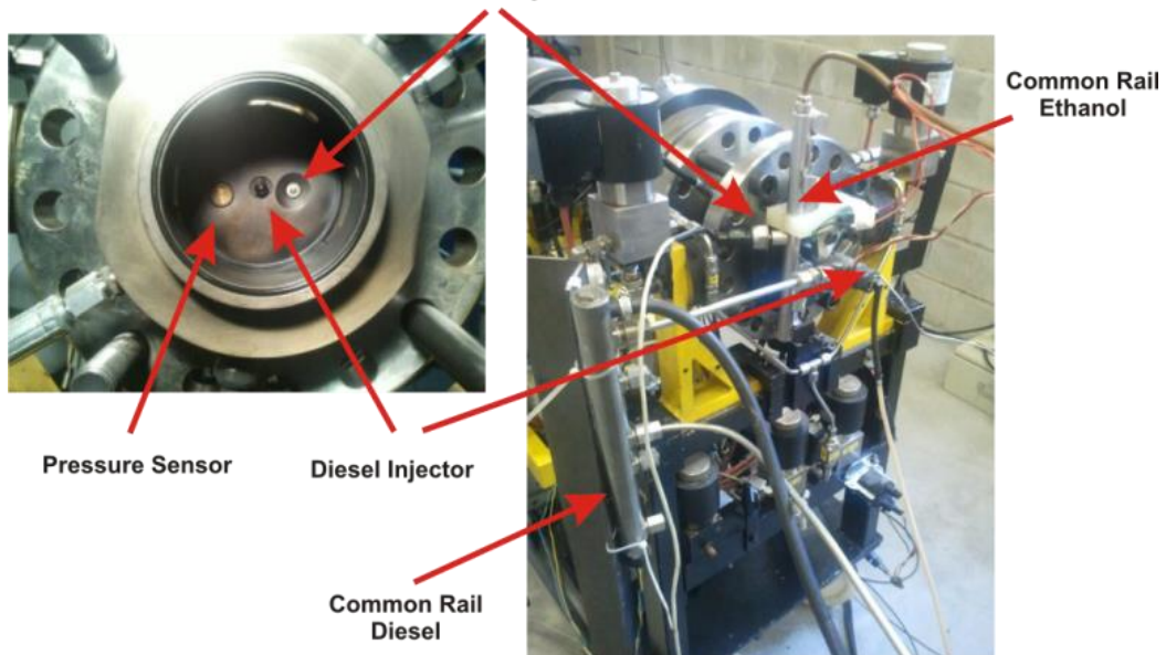
Figure 4. Adaptation system of dual fuel injection in MCR. Ethanol Injector
