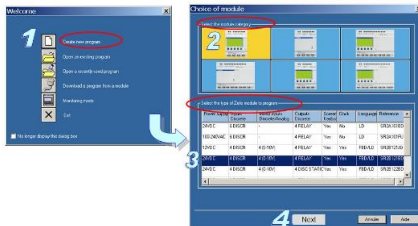
Figura 1 – Software Zeliosoft 2.
