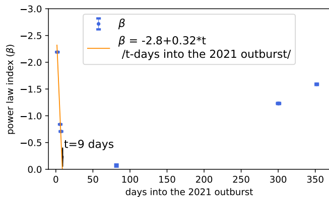
Fig. 7. Long-term variability of the index of the power law fit, \beta , to the polarization degree dependence with wavelength.
