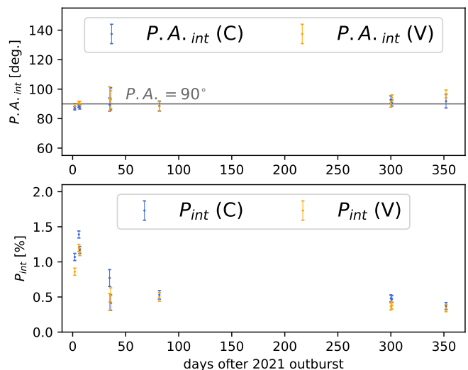
Fig. 8. Long-term variability of the position angle (top) and degree of intrinsic polarization (bottom) of RS Oph after the start of the 2021 outburst. The P.A. was practically constant throughout our observing campaign, while the degree of intrinsic polarization reached a maximum at day 5.9 and has been decreasing since then.
