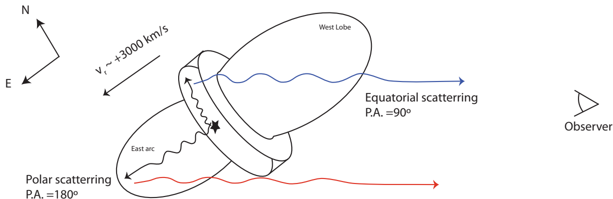
Fig. 10. Schematic view of the polar and equatorial scattering regions that are detected at different position angles and their contribution to the polarized flux.
