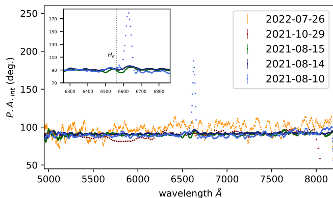
Fig. 6. Intrinsic position angle of RS Oph after the 2021 outburst. Aside from the 180^\circ position angle around the H\alpha region on day 2, the position angle of the intrinsic polarization is on average 90^\circ , implying that the scattering region that produced the observed polarization was oriented perpendicular to the elongated structures observed at other wavelengths during the last two outbursts. The data were smoothed with a moving average over seven points to better illustrate the position angle structures.
