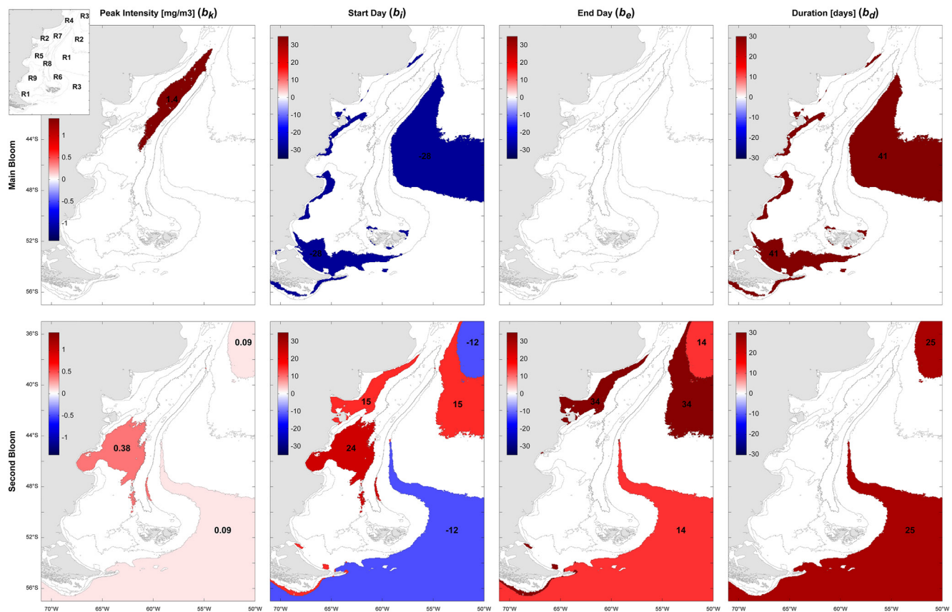
Figure 5. Trends of main and secondary phenological indices. b_k is presented in \text{mg m}^{-3} \text{decade}^{-1} and b_i , b_e , and b_d in days \text{decade}^{-1} . Only the regions painted are statistically significant ( p < 0.05 ).
