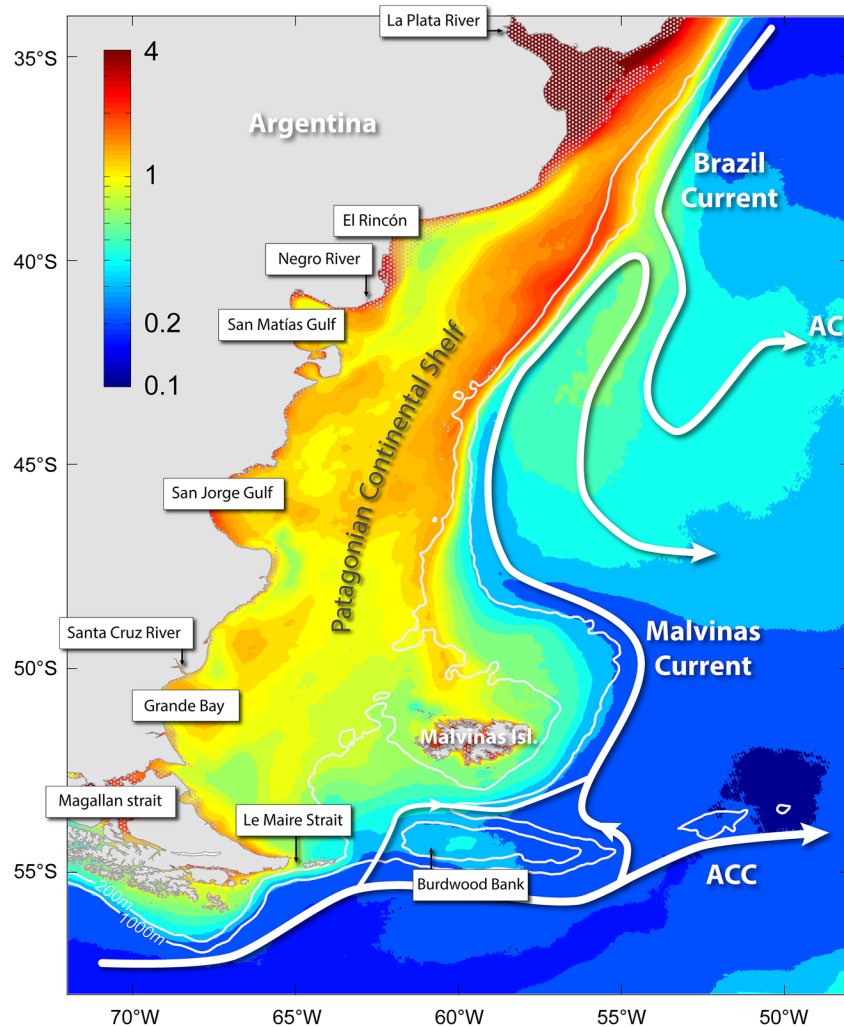
Figure 1. Mean Chlorophyll-a concentration ( \text{mg m}^{-3} ) in the Southwestern Atlantic Ocean (SWA) for the period (1998–2021) and, overlapped, main circulation patterns (thick arrows). Dotted areas (i.e., in La Plata River) indicate biased chlorophyll-a values that were excluded from the analysis.
