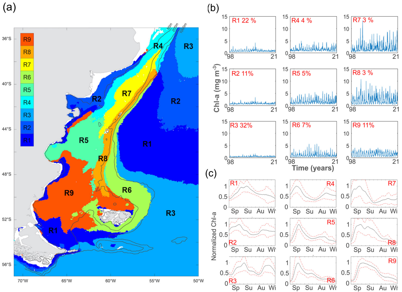
Figure 2. (a) Biogeographical classification of Chl-a depicted from the 3 \times 3 Self-Organizing Map (SOM) classification. (b) Characteristic Chl-a temporal patterns obtained from SOM computation. The inset number in red indicates the percentage of pixels clustered in each neuron. (c) Normalized climatology of the Chl-a temporal patterns. The solid black line indicates the mean and dashed red lines indicate \pm one standard deviation. Sp = Spring, Su = Summer, Au = Autumn, Wi = Winter.
