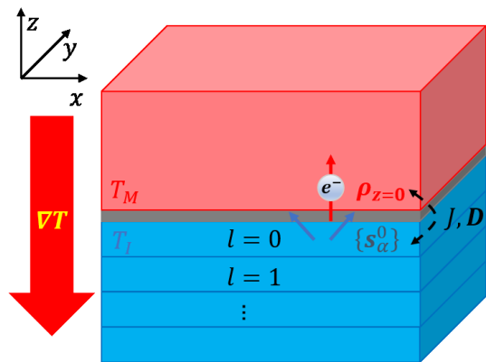
FIG. 1. (Color online.) Longitudinal Spin Seebeck setup. A thermal gradient \nabla T is applied perpendicular to the interface of the heterostructure. The upper red portion is the non-magnetic metal with temperature T_M near the interface, modeled as a degenerate Fermi gas. The lower blue part is the magnetic insulator with temperature T_I , which can be regarded as multiple two dimensional layers with layer index, l . The grey part represents the interface, where the electron spin density, \rho_{z=0} , and \alpha -th interfacial magnetic moments, \mathbf{S}_{\alpha}^0 , are coupled with an isotropic Heisenberg exchange J and DM interaction D .
