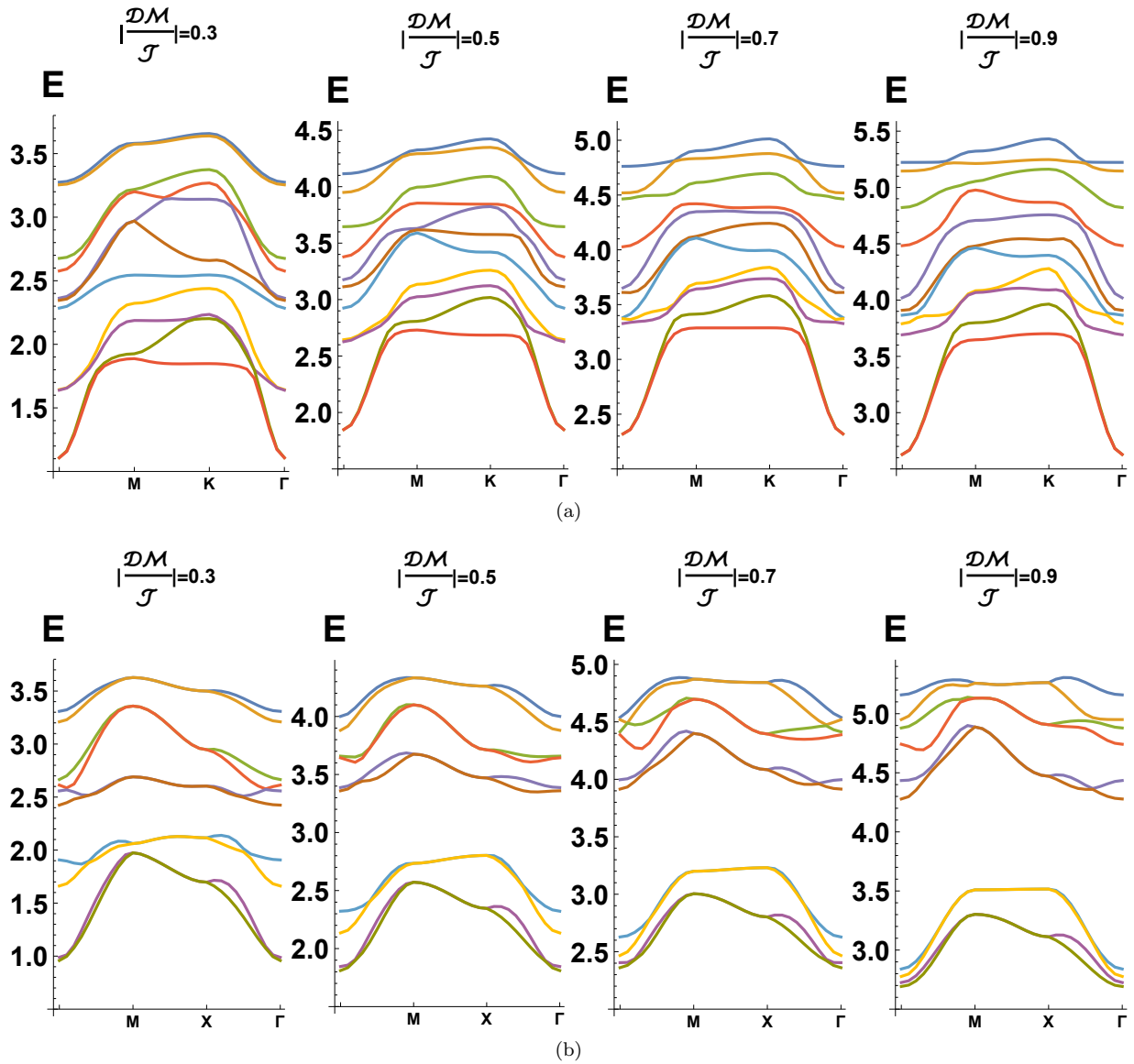
FIG. 3. (Color online.) Bulk magnon spectrum along high symmetry directions for different crystalline orientations. |\frac{DM}{J}| is the ratio between the exchange interaction and DMI in the bulk. Energies are given in units of \frac{t^2}{U} . (a) Crystalline orientation along [111]. (b) Crystalline orientation along [100].
