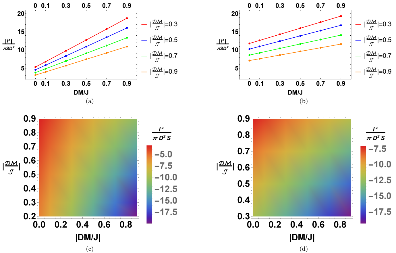
FIG. 7. (Color online.) The magnitude of z -polarized spin current density/ \pi D^2 S as a function of the coupling strength. (a) Crystal oriented in [111] and (b) Crystal oriented in [100]. (c)(d) Corresponding density plots for [111] and [100] orientation. Here k_B T_M = 5J/8 and k_B T_I = J/2 , J_{ij} = J , |\frac{DM}{J}| is the coupling ratio in the bulk and |\frac{DM}{J}| is the coupling ratio at the interface. S is the magnitude of the local spin and the effective S=1/2 in PI.
