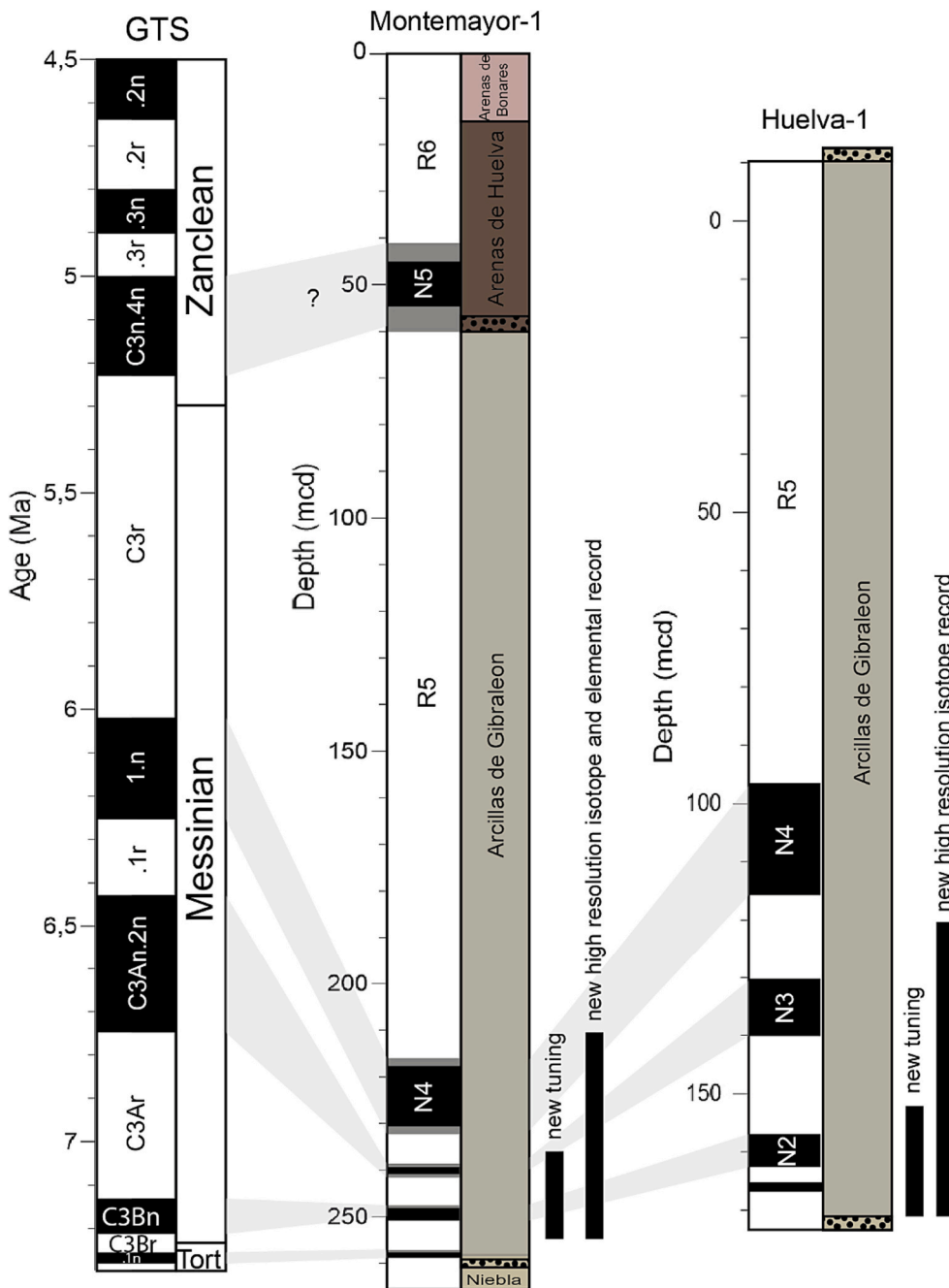
Fig. 2. On the left, the Tortonian – Zanclean magnetostratigraphic chrons from Lourens et al. (2004). In the Middle the magnetostratigraphic results for Montemayor-1 core (Larrasoña et al., 2008; Larrasoña et al., 2014) and the lithological column showing the different formations present in Montemayor-1 core (Niebla Formation, Arcillas de Gibralfaleón Formation, Arenas de Huelva Formation and Arenas de Bonares Formation). On the right, the magnetostratigraphic results for Huelva-1 core (Larrasoña et al., 2008; Larrasoña et al., 2014) and the lithological column showing the different formations present (Arcillas de Gibralfaleón Formation).
