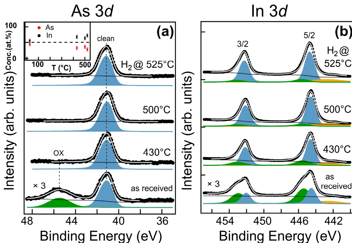
Figure 2. XPS spectra of the As 3d (a) and In 3d (b) core level regions of as-received InAs nanowires (bottom), after annealing at 430 °C, 500 °C and after H _2 pre-treatment at 525 °C (top) and corresponding fits. The inset shows the As (red) and In (black) concentrations after the same three pre-treatments. The dotted line corresponds to stoichiometric InAs (50%). The green and blue components refer to, respectively, oxidized and non-oxidized InAs-related components, while the yellow component is due to the MgK \alpha satellites (see text for more details).
