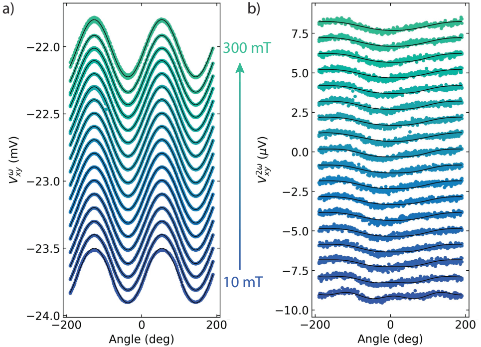
Figure 5.6: (a) First-harmonic and (b) second-harmonic Hall signals obtained for a device fabricated using regular lithography techniques for various magnetic field strengths. For this device, the WSe 2 has been in contact with the e-beam resist PMMA prior to the evaporation of permalloy. No significant deviations from the \sin(2\phi) were observed in the first-harmonic Hall signal down to 10 mT fields, indicating little or no magnetic anisotropy. No field dependence was observed for the second-harmonic Hall signal, indicating the absence of measurable spin-orbit torques. The modulation of the second-harmonic Hall voltage is ascribed to the anomalous Nernst effect.
