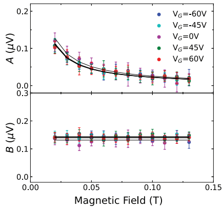
Figure 5.5: The A- and B-component (according to Eqs. 5.3 and 5.4) as a function of magnetic field for different gate voltages for device D_4^B .
