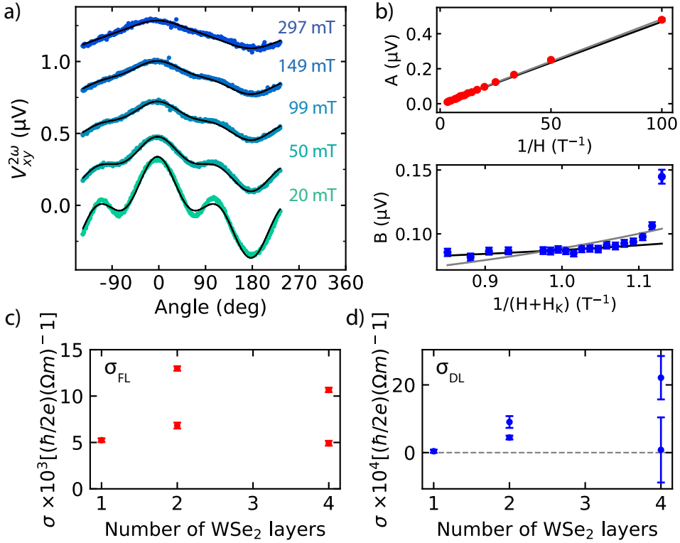
Figure 5.2: (a) Second-harmonic Hall measurements at various magnetic fields for one WSe 2 /Py device D_2^A . The colored circle represent the data while the black line are fits using Eq. 5.2. The measurements for different fields have been offset for clarity. (b) The A- and B-component extracted from the fit of (a) for various magnetic field strengths. The straight lines corresponds to the fits using Eqs. 5.3 and 5.4. The grey line corresponds to the fit using the data points from all magnetic fields, while the black line corresponds to the fit for fields starting at 40 mT. The error bars are obtained from the standard deviation from the fit. (c, d) The spin-torque conductivities of the (c) field-like and (d) antidamping-like torque, calculated using Eq. 5.5, for devices with various WSe 2 thickness.
