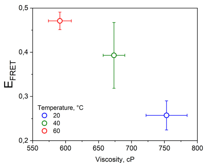
Figure 7. Fusion inversely scales with viscosity as assessed upon temperature shifts. Lo GUVs made of DPPC:DPPG:Chol (2:5:3 mol ratio) were labeled with 0.5 mol% of either Bodipy C 12 or Bodipy C 16 for the fluidity and FRET experiments, respectively. In the fusion experiments, the GUVs were incubated with 15 \mu M LUVs (total lipids) labeled with 2 mol% DPPE-Rh. The data display the mean and SEMs for viscosity and E_{\text{FRET}} . DPPC, 1,2-dipalmitoyl-sn-glycero-3-phosphocholine; DPPE-Rh, 1,2-dipalmitoyl-sn-glycero-3-phosphoethanolamine-N-(lissamine rhodamine B sulfonyl); DPPG, 1,2-dipalmitoyl-sn-glycero-3-phospho-(1'-rac-glycerol); GUV, giant unilamellar vesicle; LUV, large unilamellar vesicle.
