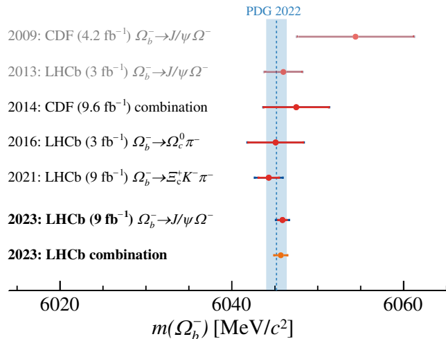
FIG. 2. Overview of the \Omega_b^- mass measurements to date (red points) [3–7], with corresponding statistical and systematic uncertainties marked in red and blue, respectively, as well as the current world average by the PDG [1] (light-blue band). The superseded measurements are shown with lighter colors. The measurement by the DØ experiment [2] of 6165 \pm 22 MeV/ c^2 is not shown, because it is inconsistent with all others and falls outside the range of this plot. The new LHCb combination is presented in orange, where the total uncertainty is shown.
