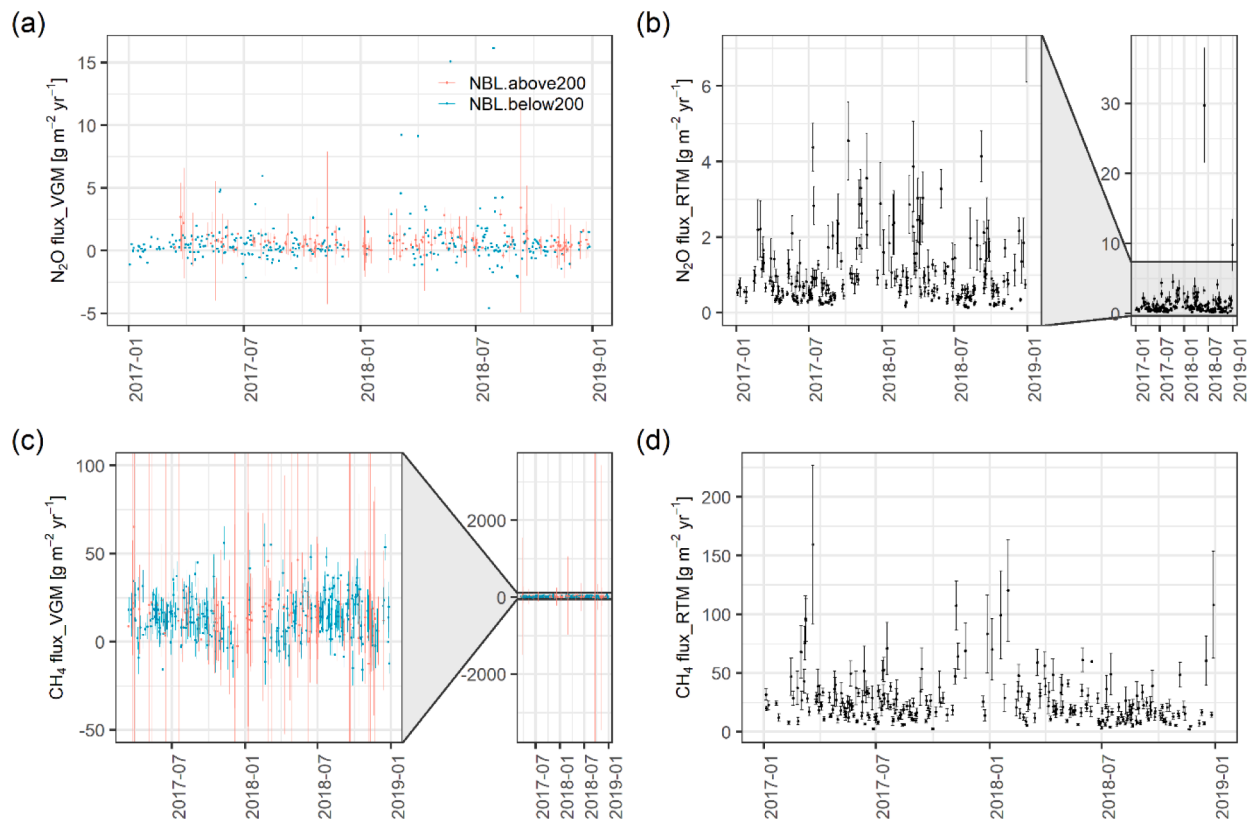
Fig. 2. Surface fluxes with uncertainties (error bars) in g\ m^{-2}\ yr^{-1} for (a) and (b) N_2O , and (c) and (d) CH_4 estimated using the VGM (left panel) and RTM (right panel). The colors indicate the VGM fluxes when the NBL height is above (red) and below (blue) 200 m. The RTM fluxes of N_2O between 0 and \sim 7\ g\ m^{-2}\ yr^{-1} and the VGM fluxes of CH_4 between -50 and \sim 100\ g\ m^{-2}\ yr^{-1} were zoomed in for clarity.
