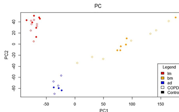
Fig. 1 Principal component (PC) analysis. PC in the RNA obtained from lung-derived MSCs (LM; red), bone marrow-derived MSCs (BM; yellow) and adipose-derived MSCs (AD; blue) from COPD patients (open circles) and controls (closed circles)
