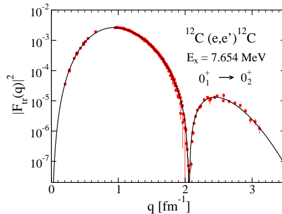
Figure 2. Squared form factor for the transition from the ground state in ^{12}\text{C} to the Hoyle state extracted by the model-independent analysis (solid line) described in the text in comparison to the experimental data [14, 17] transformed according to Eq. (2).
