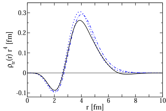
Figure 3. Transition charge density corresponding to the form factor displayed in Fig. 2 multiplied by r^4 (full line) in comparison to the theoretical predictions [18] of FMD (dotted line) and an \alpha particle gas (dashed-dotted line).
