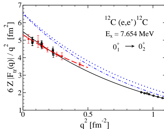
Figure 4. Experimental form factors at low q corrected by Eq. (2) compared to different model approaches. Extrapolation to zero momentum transfer provides the monopole matrix element. Square symbols and dashed line: new data and polynomial fit with Eq. (6). Circles and full line: old data and global fit with Eq. (4). Dashed-dotted line: FMD model, dotted line: \alpha -cluster model [18].
