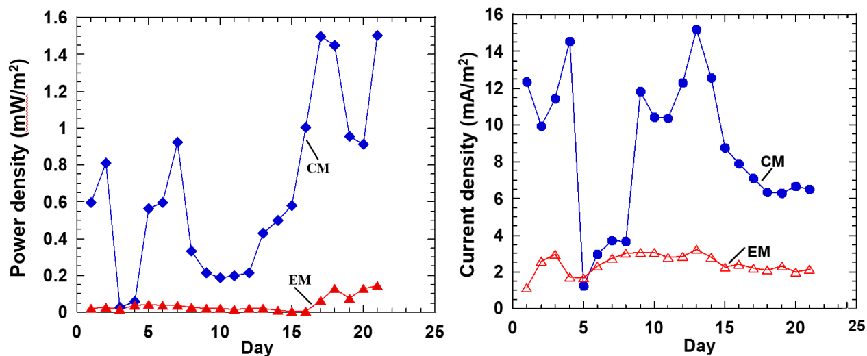
FIGURE 2. Power and current density of MFC from different bacterial sources
