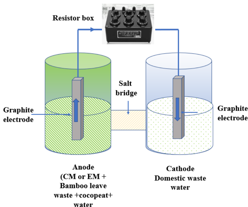
FIGURE 1. Construction of double chamber bamboo leaf MFC
