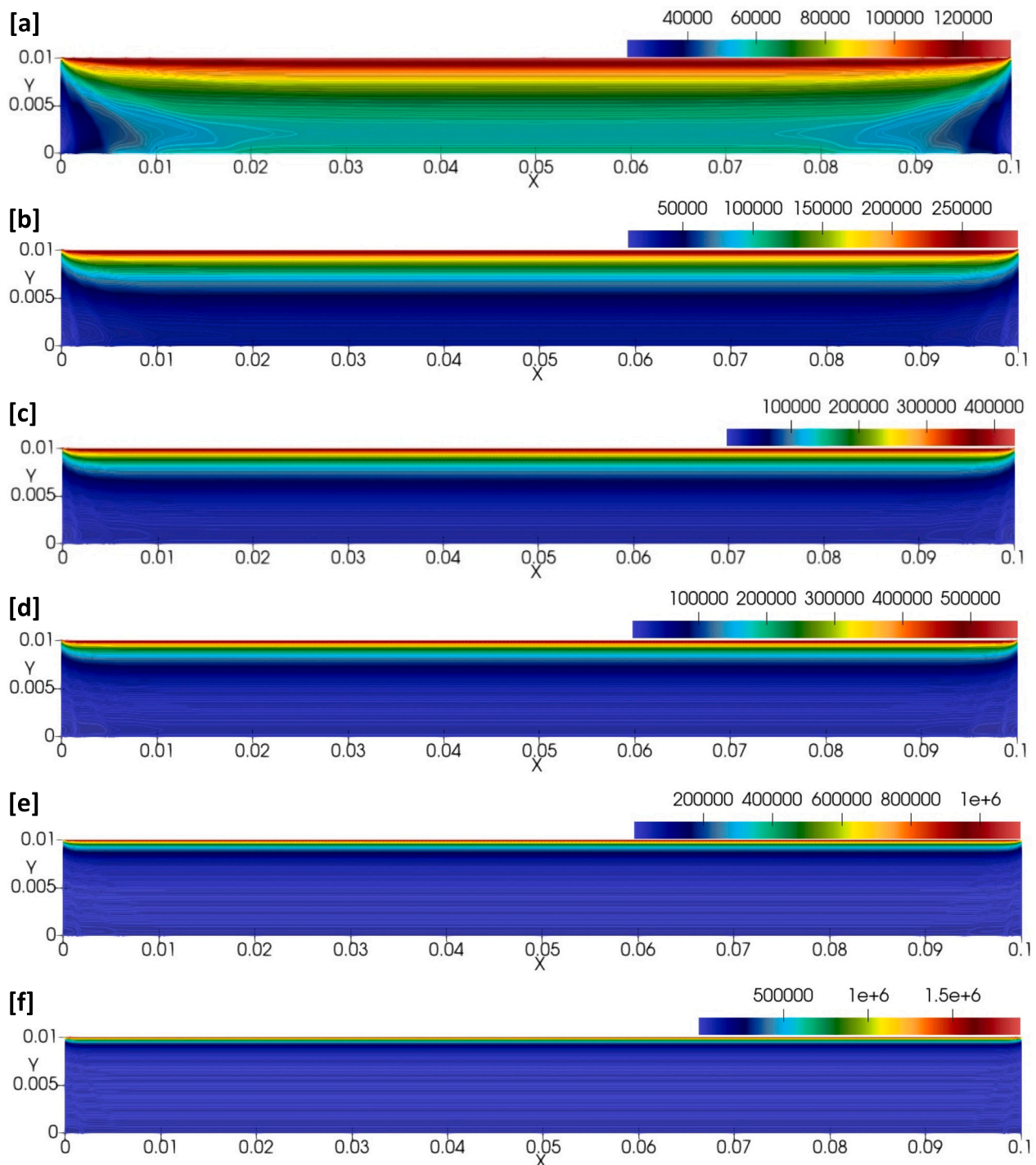
Fig. 23. Volumetric absorbed radiation ( \text{Wm}^{-3} ) profiles of paraffin/Al slurry at different shell concentrations: (a) 4, (b) 10, (c) 15, (d) 20, (e) 40, and (f) 70 ppm.
