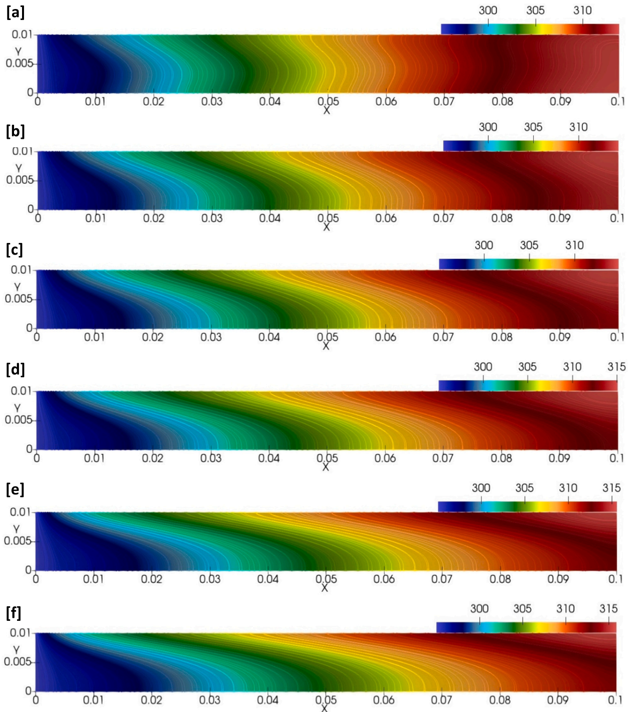
Fig. 22. Temperature (K) profiles of paraffin/Al slurry at different shell concentrations: (a) 4, (b) 10, (c) 15, (d) 20, (e) 40, and (f) 70 ppm.
