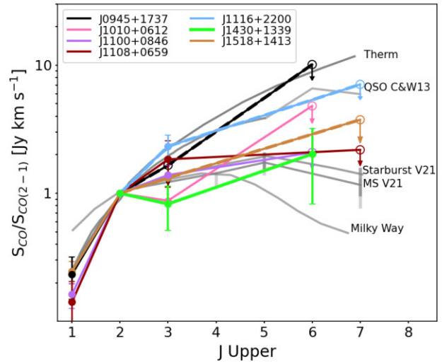
(b) For the 7 targets which have either CO(6-5) or CO(7-6) data we present the CO SLEDs up to these higher transitions. Here we are normalising to the CO(2-1). Literature comparison data showing high- z quasars Carilli & Walter (2013) (C&W13) and z = 1 - 2 Starburst and main sequence (MS) Valentino et al. (2021) (V21). 3 sigma upper limits are indicated by empty circles with downward arrows. No uncertainties are shown for CO(2-1) as these are incorporated into the uncertainties on CO(1-0), CO(3-2) and CO(6-5) to best represent the uncertainty on the excitation level.
