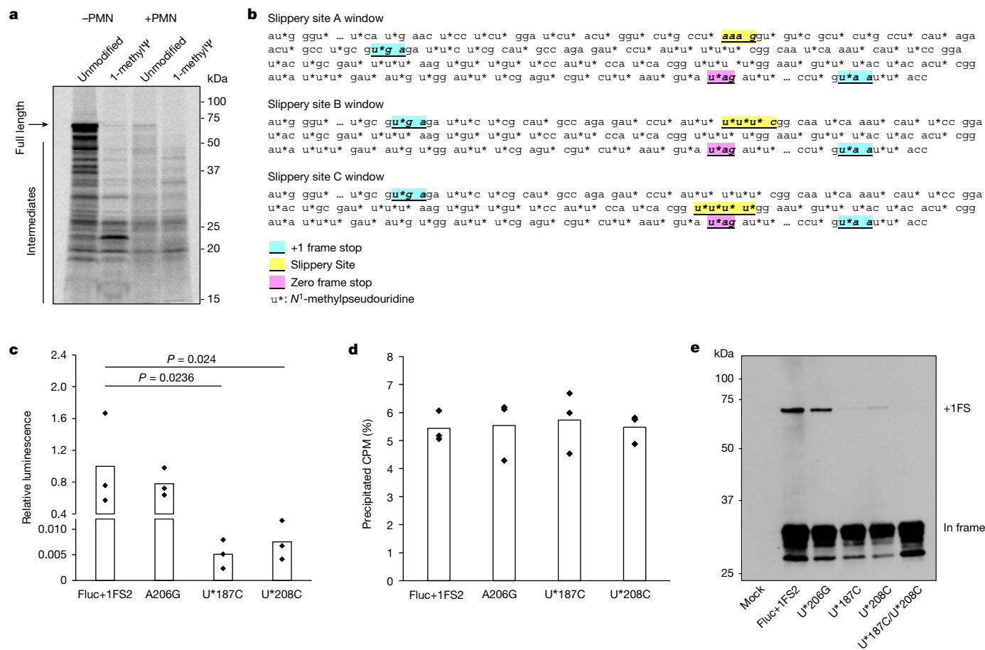
Fig. 4 | +1 ribosomal frameshifting is dependent on mRNA slippery sequences and associated with ribosome stalling during 1-methylψ mRNA translation. a , SDS–polyacrylamide gel electrophoresis autoradiograph of [ 35 S] methionine-labelled polypeptides produced by translation of unmodified or 1-methylψ Fluc mRNA for 30 min, including or omitting 100 μM paromomycin (+PMN and –PMN, respectively). b , Diagram showing putative mRNA slippery sequences and stop-codon-flanked windows. c , Activity of +1 frameshifted products after translation of 1-methylψ mutant mRNAs, or 1-methylψ Fluc+1FS2
