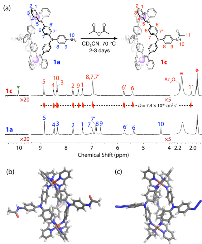
Figure 1. (a) 1 H NMR spectra (400 MHz, 298 K, CD 3 CN) of helicates 1a and 1c . The appearance of a new acetyl –CH 3 singlet at \delta = 2.02 ppm and the high symmetry of the final NMR spectrum allow us to infer efficient conversion of 1a to the acetylated helicate. Only very slight decomposition of 1a was observed, as indicated by the aldehyde signal at 10 ppm. Intensities have been scaled for clarity. Asterisks denote residual solvent peaks. (b) Cationic portion of the X-ray crystal structure of acetylated helicate 1a . (c) Cationic portion of the X-ray crystal structure of azido helicate 1n . Disorder is omitted in both structures for clarity.
