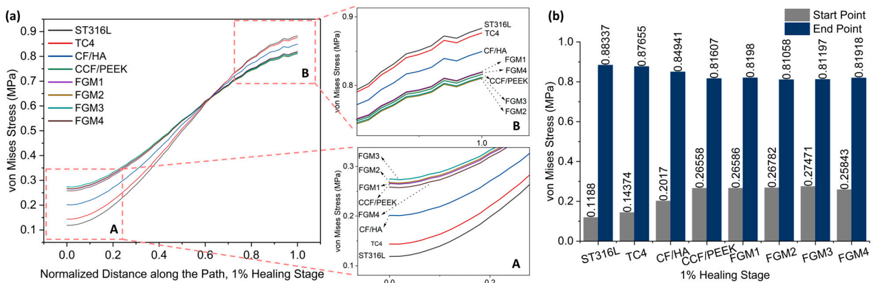
Figure 6. Von Mises stress distributions along the path for the 1% healing stage: (a) von Mises stress variation along the path; A and B are magnified views of the start point and end point area; (b) a bar chart with specific values of the start point and end point labeled on top of the bar.
