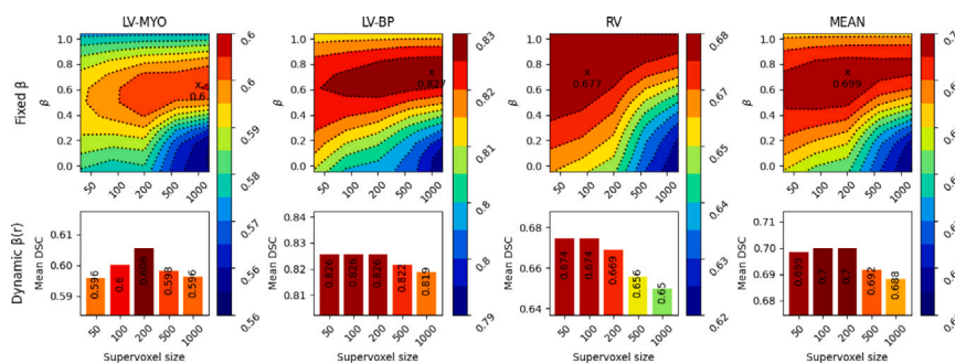
Fig. 11. Parameter sensitivity of feature-refinement module on the MS-CMRSeg dataset. Top: Grid-search over supervoxel sizes and a range of fixed betas. Bottom: Line-search over supervoxel sizes with a dynamic beta automatically computed from uncertainty maps.
