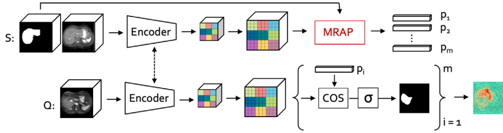
Fig. 1. We facilitate the estimation of uncertainty maps in prototypical FSS models by replacing the deterministic masked average pooling module with a randomized alternative, the masked randomized average pooling (MRAP), denoted in red. This allows us to generate a set of prototypes, and thereby a set of query predictions that can be used to estimate the model uncertainty.
