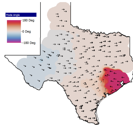
Figure 8: Visualization of 0.63 Hz Southeast Mode
