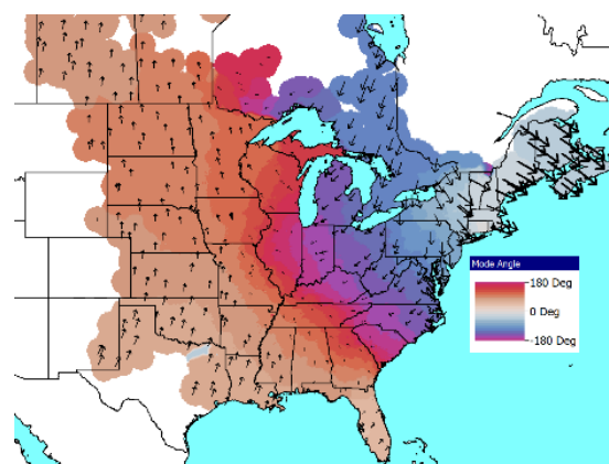
Figure 27: NEng Forced Oscillation 0.27 Hz Mode Shape
