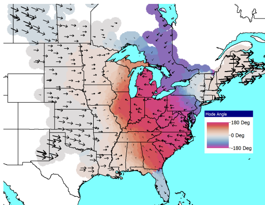
Figure 25: Northeast Disturbance, 0.35 Hz Mode Shape, 15.0% Damping
