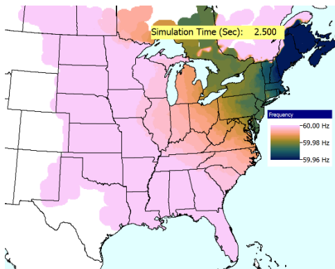
Figure 15: Spatial Frequency for the Figure 14 Scenario at 2.5 Seconds
