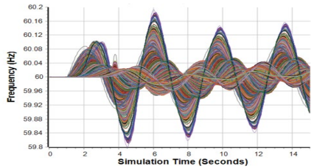
Figure 26: Frequencies of 0.27 NEng Forced Oscillation
