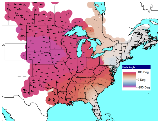
Figure 20: Nebraska Scenario, 0.25 Hz Mode Shape, 20.2% Damping
