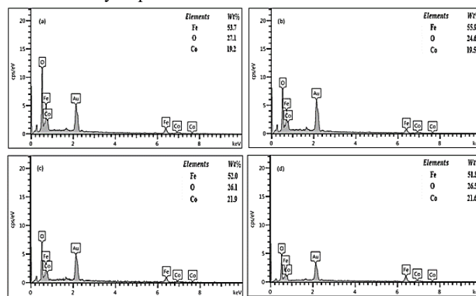
Fig 4: EDS spectra of \text{Co}_{1.2}\text{Fe}_{1.8}\text{O}_4 nanoferrites for (a) as-burnt (b) calcined sample at 500°C (c) at 600 °C and (d) at 700 °C.
