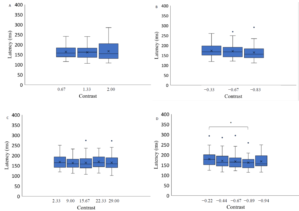
Figure 4. Saccadic eye movement latency as a function of stimulus contrast on three backgrounds (medium grey (positive (A) and negative (B) polarity), black (C) and light grey (D)). Data outliers, which are significantly different from the rest of the data, are marked with dots. * indicates statistically significantly different results after pairwise comparisons (post hoc analysis) with Bonferroni correction p -value < 0.05 (SPSS).
