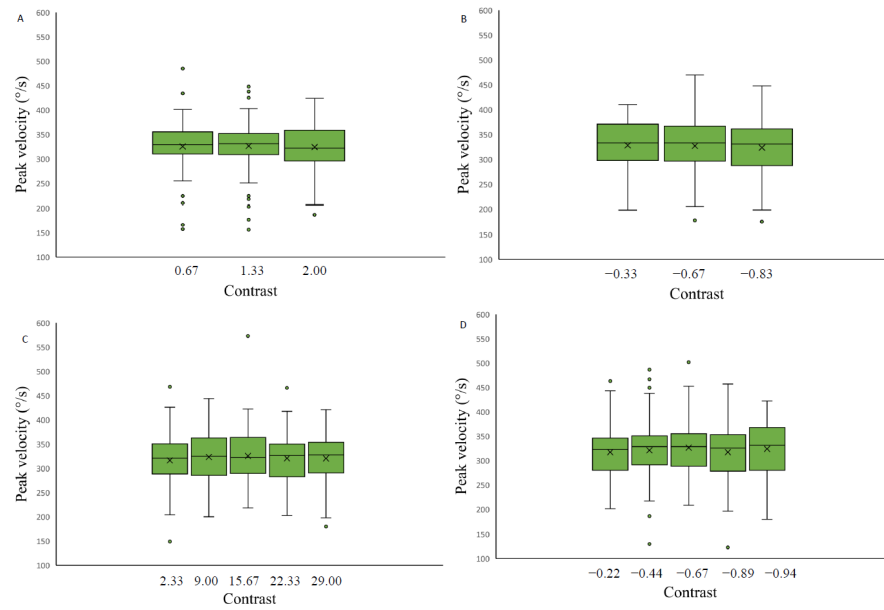
Figure 8. Saccadic peak velocity as a function of stimulus contrast on three backgrounds (medium grey (positive (A) and negative (B) polarity), black (C) and light grey (D)). Data outliers, which are significantly different from the rest of the data, are marked with dots.
