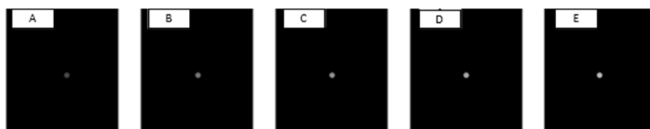
Figure 3. Saccadic eye movement targets on a black background ( 3 \text{ cd/m}^2 ). Five positive polarity contrast levels (Weber's contrast values: (A) 2.33; (B) 9.00; (C) 15.67; (D) 22.33; (E) 29.00).
