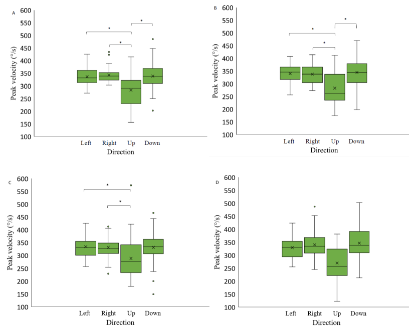
Figure 9. Saccadic peak velocity as a function of stimulus spatial position on three backgrounds (medium grey (positive (A) and negative (B) polarity), black (C) and light grey (D)). Data outliers, which are significantly different from the rest of the data, are marked with dots. * indicates statistically significantly different results after pairwise comparisons (post hoc analysis) with Bonferroni correction p\text{-value} < 0.05 (SPSS).
