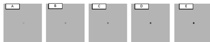
Figure 2. Saccadic eye movement targets on a light grey background (90 cd/m 2 ). Five negative polarity contrast levels (Weber's contrast values: (A) −0.22; (B) −0.44; (C) −0.67; (D) −0.89; (E) −0.94).
