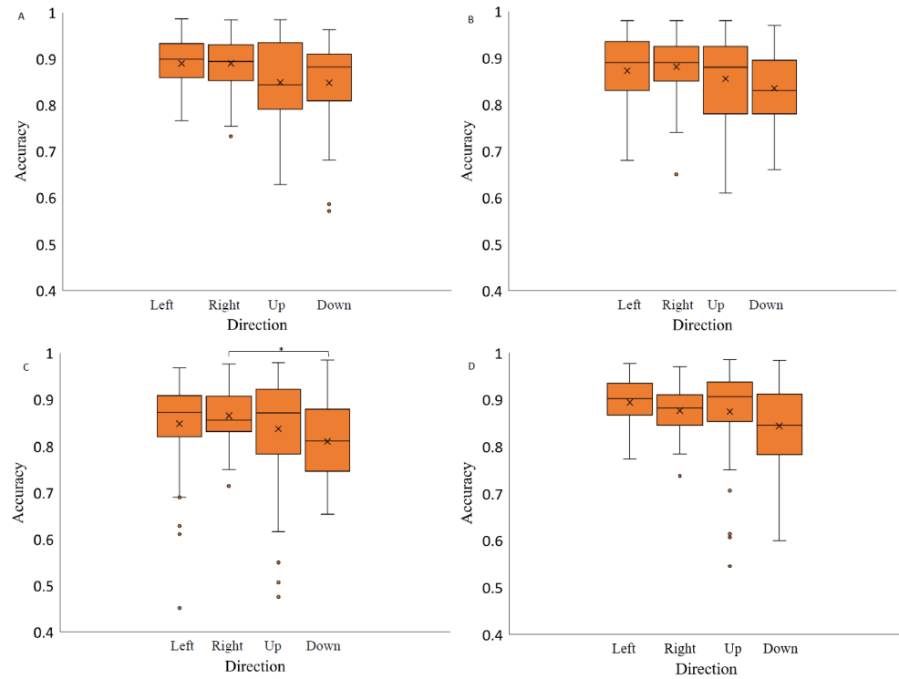
Figure 7. Saccadic accuracy as a function of stimulus spatial position on three backgrounds (medium grey (positive (A) and negative (B) polarity), black (C) and light grey (D)). Data outliers, which are significantly different from the rest of the data, are marked with dots. * statistically indicates significantly different results after pairwise comparisons (post hoc analysis) with Bonferroni correction p -value < 0.05 (SPSS).
