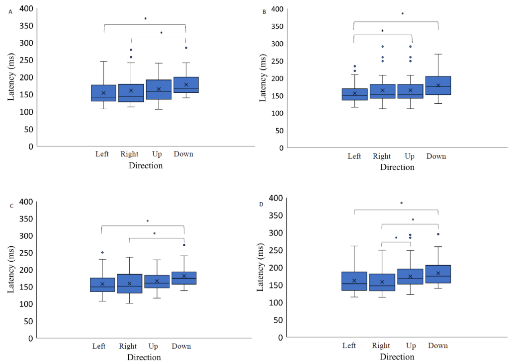
Figure 5. Saccadic eye movement latency as a function of stimulus direction on three backgrounds (medium grey (positive (A) and negative (B) polarity), black (C) and light grey (D)). Data outliers, which are significantly different from the rest of the data, are marked with dots. * indicates statistically significantly different results after pairwise comparisons (post hoc analysis) with Bonferroni correction p -value < 0.05 (SPSS).
