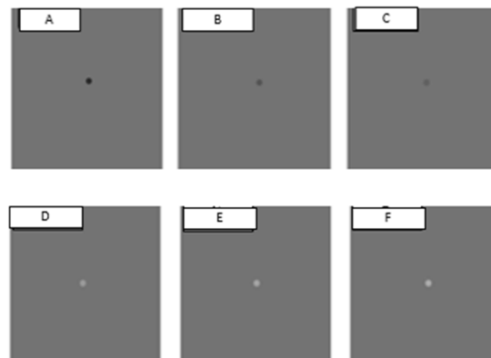
Figure 1. Saccadic eye movement targets presented on medium grey background (30 cd/m 2 ). Three negative polarity contrast levels (Weber's contrast values: (A) −0.83; (B) −0.67; (C) −0.33) and three positive polarity contrast levels (Weber's contrast values: (D) 0.67; (E) 1.33; (F) 2.00).
