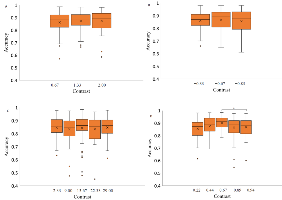
Figure 6. Saccadic accuracy as a function of stimulus contrast on three backgrounds (medium grey (positive (A) and negative (B) polarity), black (C) and light grey (D)). Data outliers, which are significantly different from the rest of the data, are marked with dots. * statistically indicates significantly different results after pairwise comparisons (post hoc analysis) with Bonferroni correction p -value < 0.05 (SPSS).
