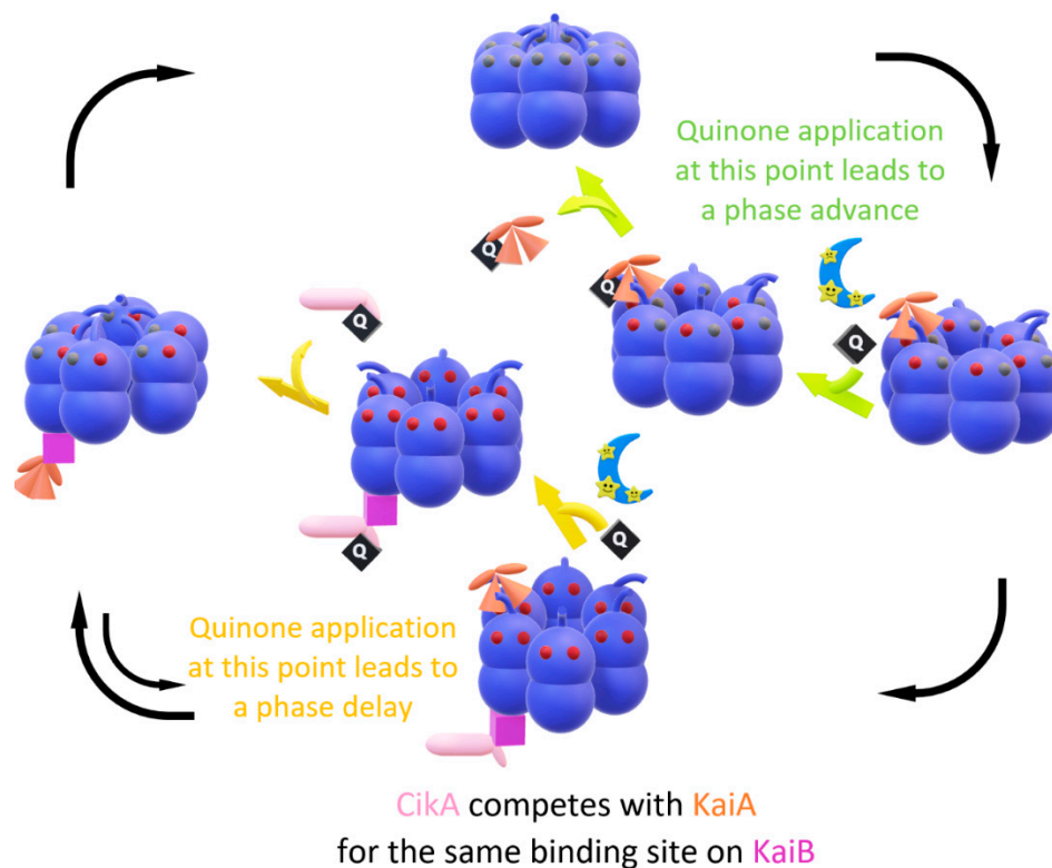
Figure 4. Schematic diagram of quinone entrainment. Oxidized quinone (“Q” in a black rhombus) becomes acutely abundant at night as a proxy for darkness. As KaiC autophosphorylation takes place, quinone application at this point inactivates KaiA, leading to premature dephosphorylation and a phase advance (lime arrows). On the other hand, in the in vitro mixture containing CikA and KaiABC, as fully phosphorylated KaiC enters the autodephosphorylating phase, quinone application at this point inactivates CikA, adding an extra time frame for the KaiA sequestration to take place, delaying the phase (yellow arrows).
