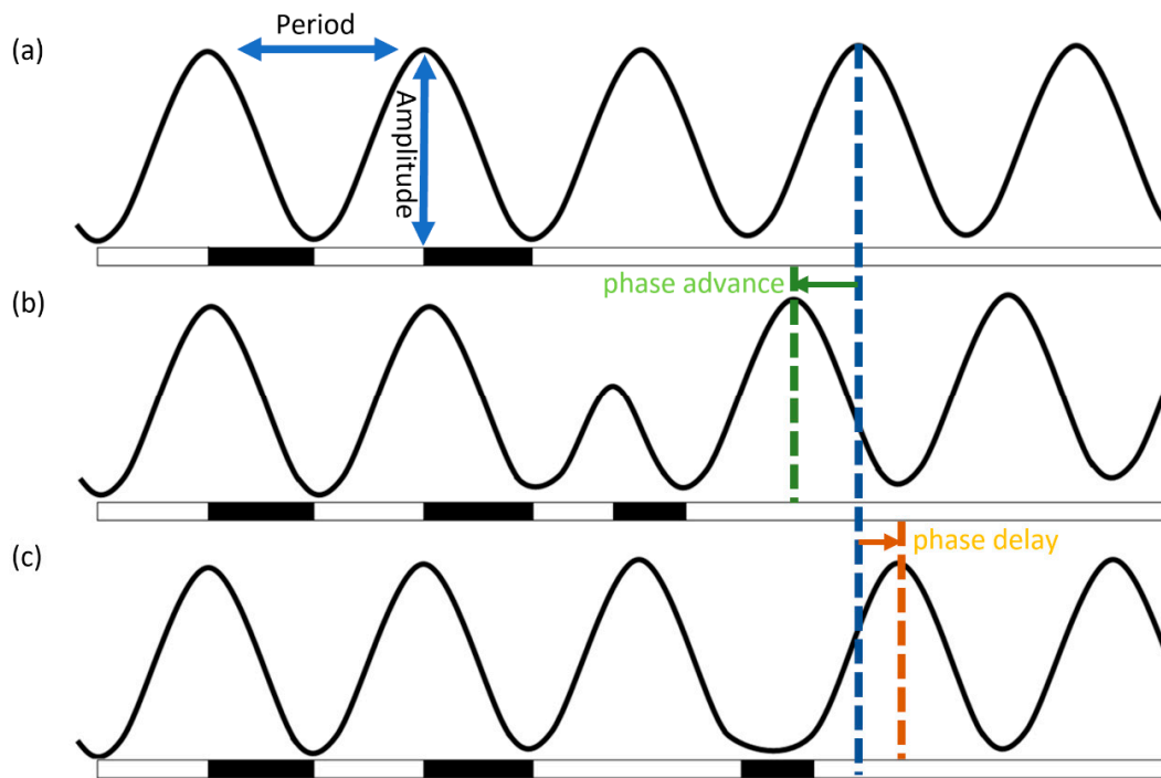
Figure 3. The entrainment of a circadian rhythm with a dark pulse. The white part on the x-axis represents light or daytime; the dark area represents either the application of a dark pulse in vivo or the application of ADP or oxidized quinone in vitro. The y-axis represents the circadian gene expression pattern or KaiC phosphorylation rhythm in cyanobacteria. (a) A free-running rhythm that still runs even under a continuous light condition. (b) A phase advance that is caused by a dark-related cue during the rising phase of the clock. (c) A phase delay that is caused by a dark-related cue during the falling phase.
