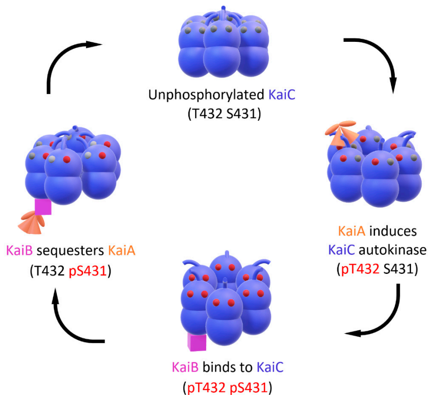
Figure 2. Ordered phosphorylation and dephosphorylation of KaiC. The initial unphosphorylated KaiC hexamer has the A-loops in their buried conformation by default. KaiA's binding tethers the A-loops in their exposed conformation, initiating autokinase activity and phosphorylating T432 first. Then, KaiC reaches its fully phosphorylated state by phosphorylating its remaining S431. At this point, KaiC's affinity for KaiB greatly increases due to their conformational changes [19,20]. KaiC–KaiB complexation ensues, sequestering KaiA away from the A-loop; the A-loops' burial leads to the dephosphorylation of T432. Through further dephosphorylation, the KaiC hexamer returns to its unphosphorylated state.
