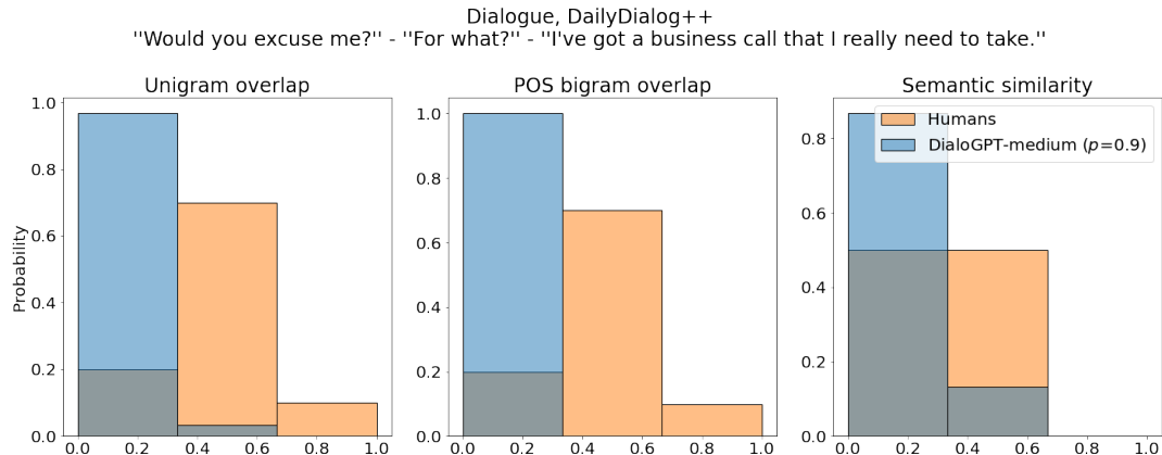
Figure 10.8: An example of variability overestimation in open-domain dialogue. Cross-variability, D_{W_1}(C_k(x), H_k(x)) , DialoGPT Medium with nucleus sampling.
