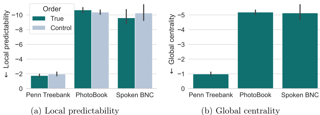
Figure 7.2: Per-document uniformity of contextualised surprisal H(S|C) . Bootstrapped 95% confidence intervals.
