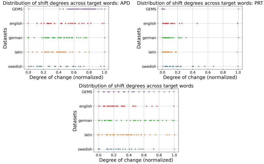
Figure 4.6: Bottom: distribution of semantic change degree in the gold data; top left: distribution of scores predicted by the APD algorithm; top right: distribution of scores predicted by the PRT algorithm.
