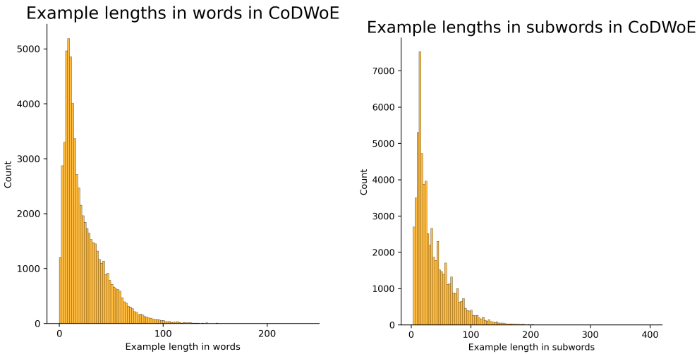
Figure A.3: Length distribution of usage examples in CoDWoE.
