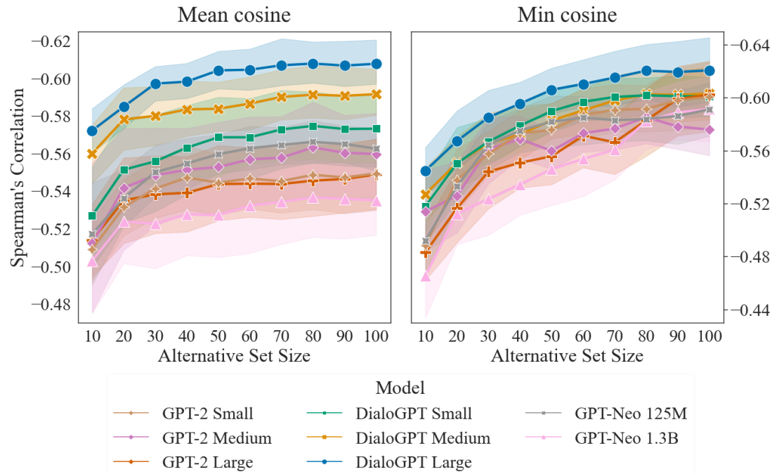
Figure 11.1: Spearman correlation between semantic information value and mean acceptability judgements in SWITCHBOARD. Confidence intervals display variability over 11 sampling strategies.
