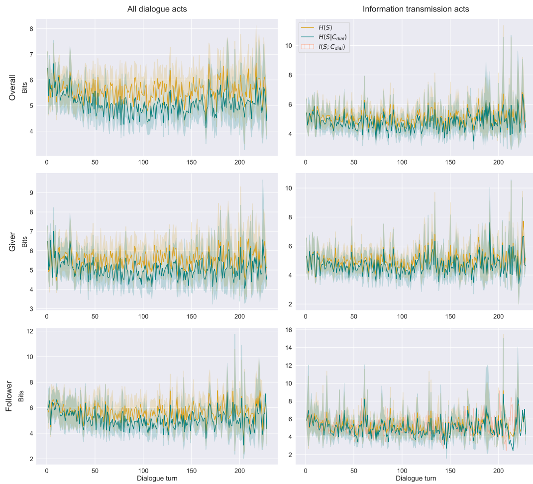
Figure 7.3: Map Task, surprisal vs. utterance position in dialogues.
