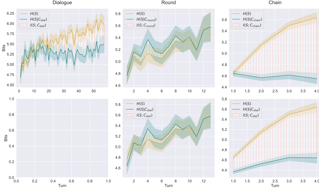
Figure 7.6: PhotoBook, surprisal vs. utterance position. All contextual units.
