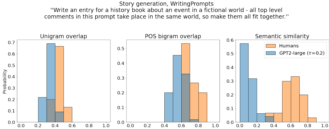
Figure 10.9: An example of variability overestimation in story generation. Cross-variability, D_{W_1}(C_k(x), H_k(x)) , GPT-2 Large with typical sampling.
