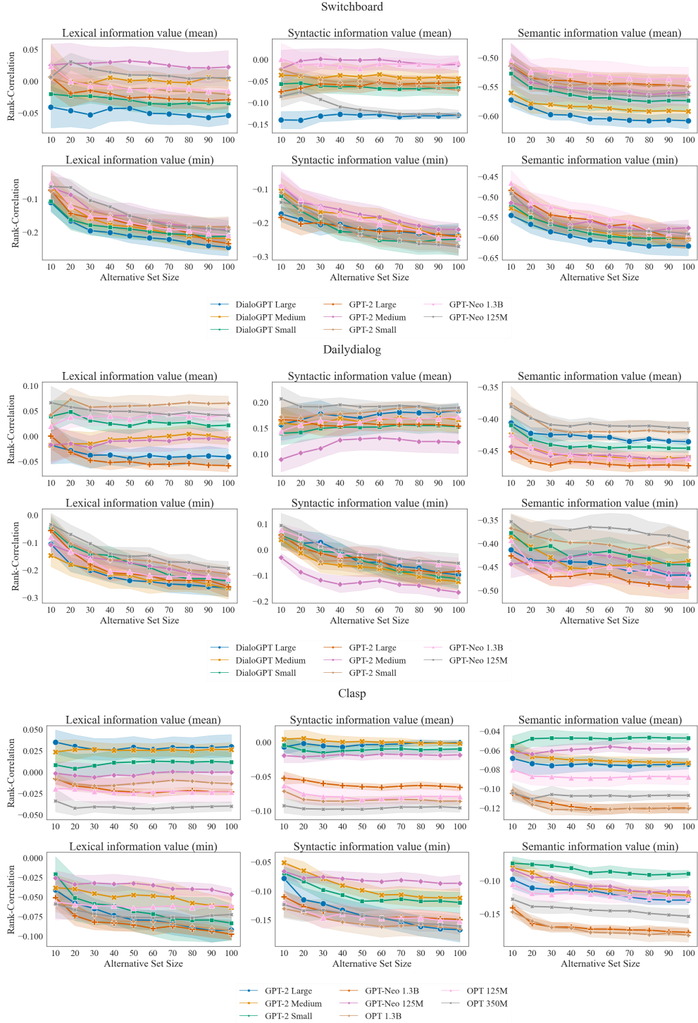
Figure C.6: Spearman correlation between information value and average acceptability judgements.
