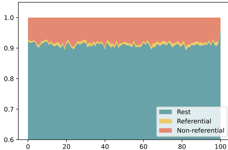
Figure 8.1: Proportion of tokens in an utterance that belong to referential constructions, non-referential constructions, and to non-construction sequences. The x axis shows percentages indicating utterance positions in the dialogue relative to the dialogue length.
