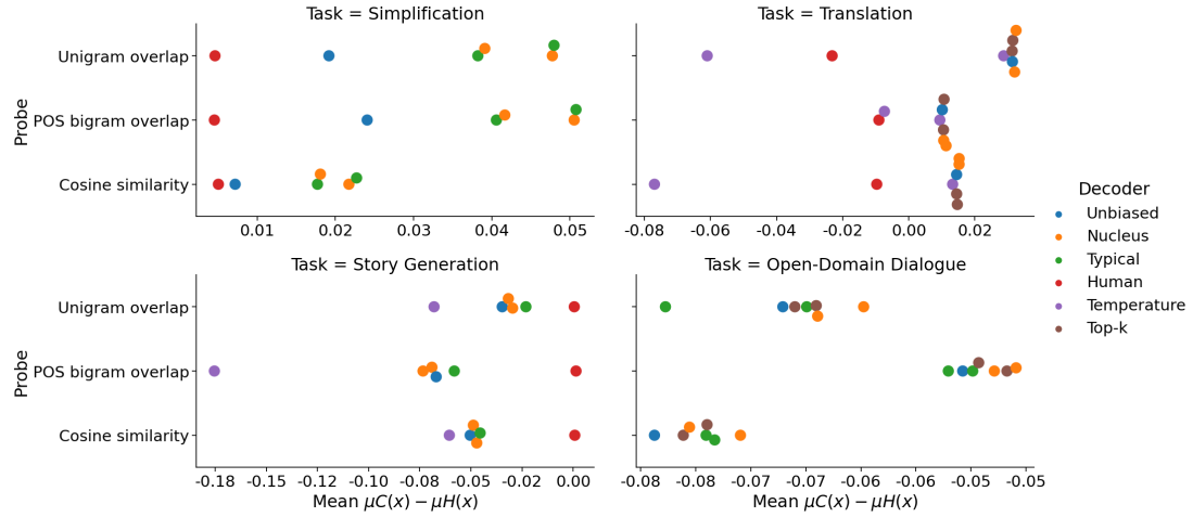
Figure C.5: Mean of distances \mu_{C(x)} - \mu_{H(x)} for (tasks, probe, decoding algorithm) tuples across test sets. Base models for each task are described in Section 10.3. Tuples that share colour have different decoding parameters.
