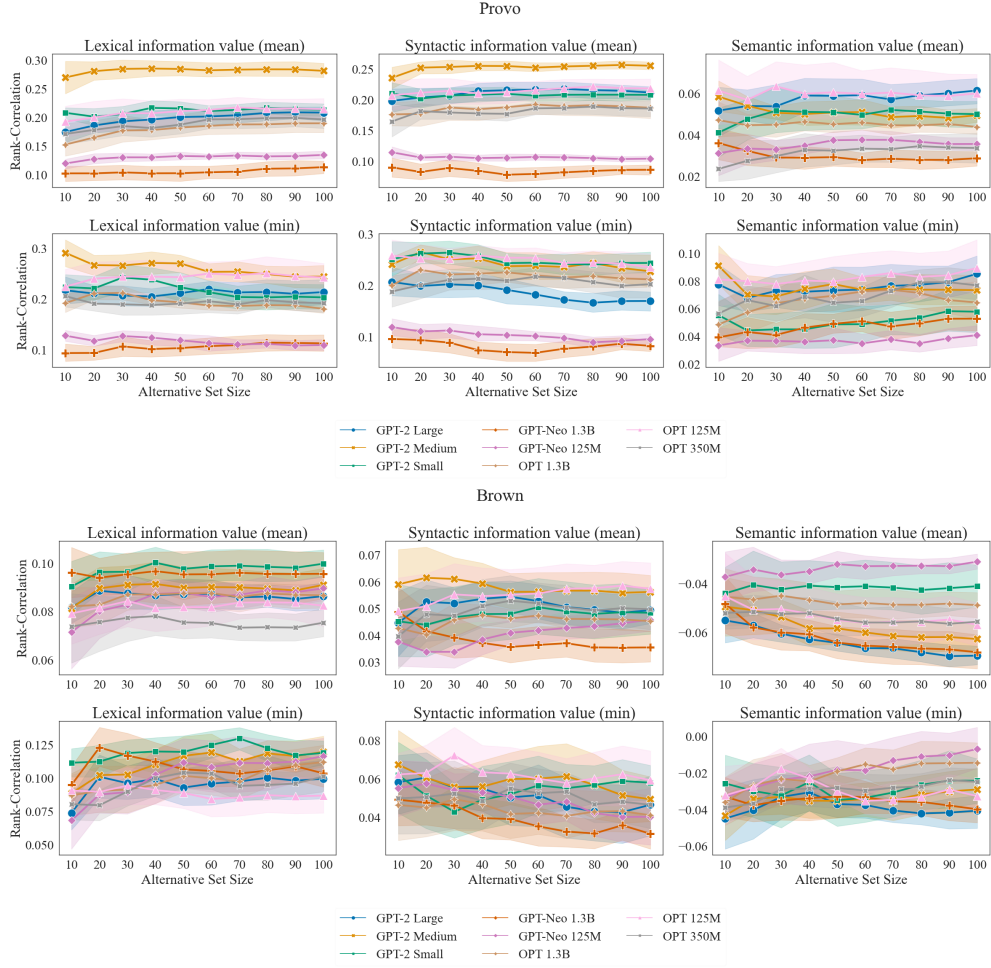
Figure C.7: Spearman correlation between information value and average reading times (length-normalised).
