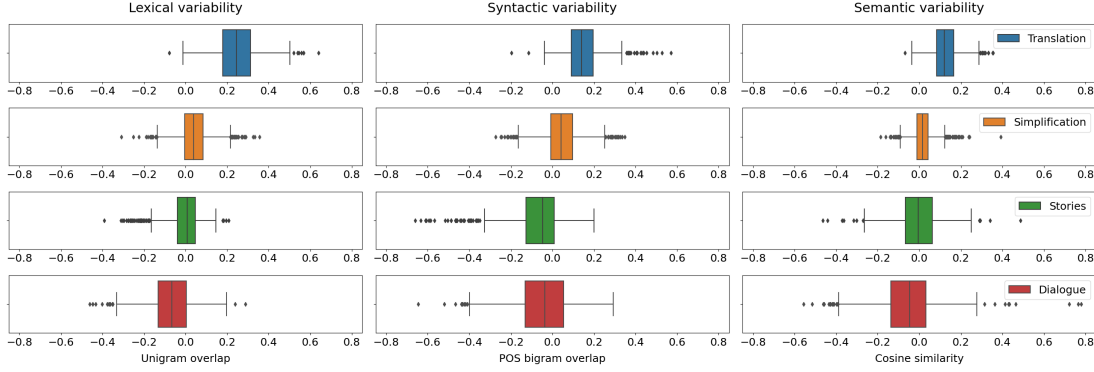
Figure 10.3: Distribution of \mu_{M_k(x)} - \mu_{H_k(x)} over instances. Values greater than zero indicate that the model underestimates the variability of the task (higher mean pairwise similarity); values below zero indicate variability overestimation.
