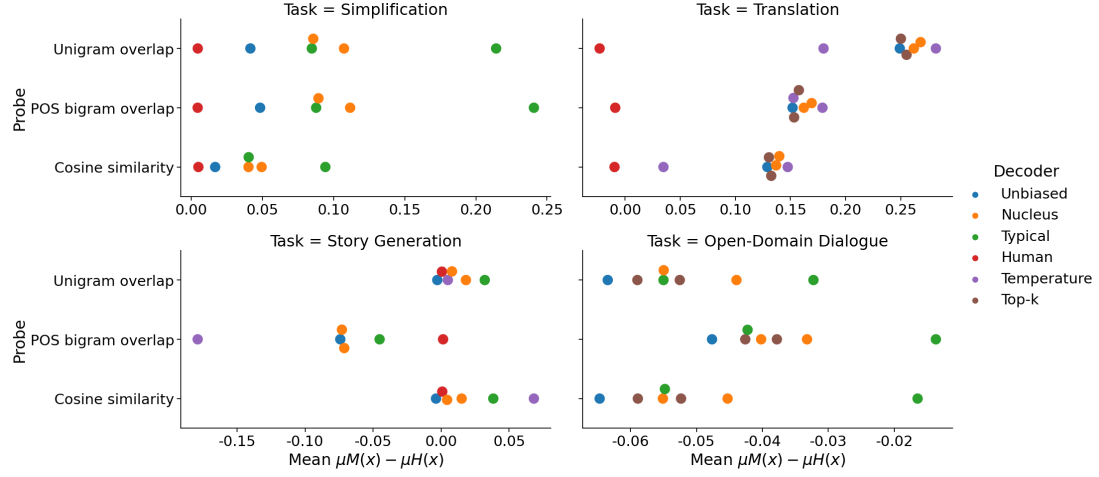
Figure C.4: Mean of distances \mu_{M(x)} - \mu_{H(x)} for (tasks, probe, decoding algorithm) tuples across test sets. Base models for each task are described in Section 10.3. Tuples that share colour have different decoding parameters.
