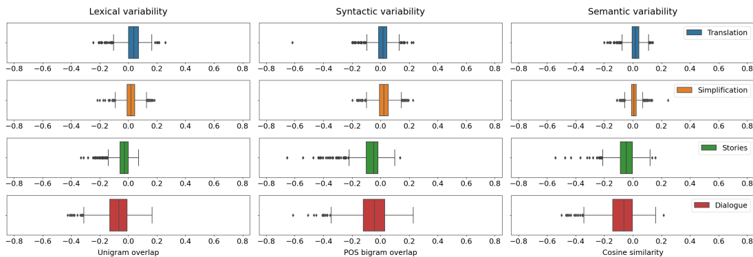
Figure 10.4: Distribution of \mu_{C_k(x)} - \mu_{H_k(x)} over instances. Values greater than zero indicate that the model underestimates the variability of the task (higher mean pairwise similarity); values below zero indicate variability overestimation.
