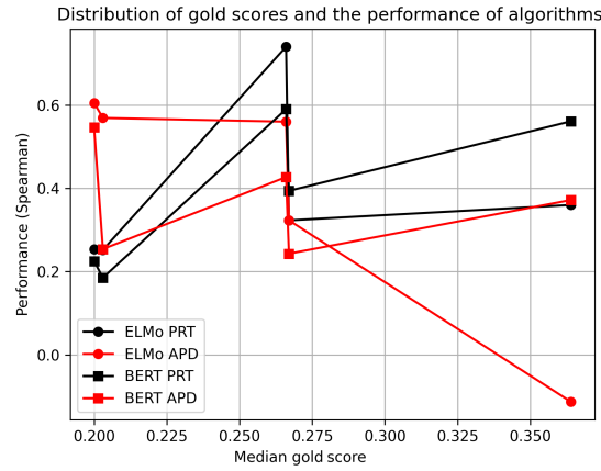
Figure 4.7: Performance of the PRT and APD algorithms depending on the median gold score.
