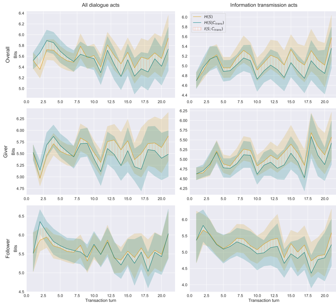
Figure 7.4: Map Task, utterance position in transactions.
