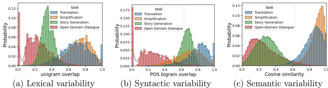
Figure 10.2: Human production variability across four NLG tasks. The values on the horizontal axis are single samples of lexical, syntactic, or semantic similarity between two productions for each input (see Section 10.2). Probability mass on the right side signals high similarity and low variability, and vice versa. A large spread indicates that production variability varies widely across inputs.
