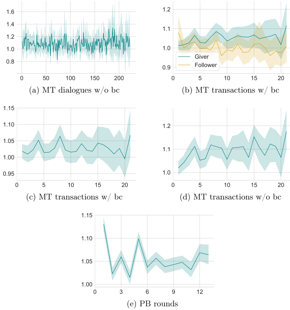
Figure B.2: surprisal ( y axis) against turn position ( x axis) in MapTask (MT) dialogues and transactions—with or without backchannels (w/ bc and w/o bc, respectively)—and PhotoBook (PB) dialogue rounds. Position is cut off at mean + 1 sd. Bootstrapped 95% confidence bands.
