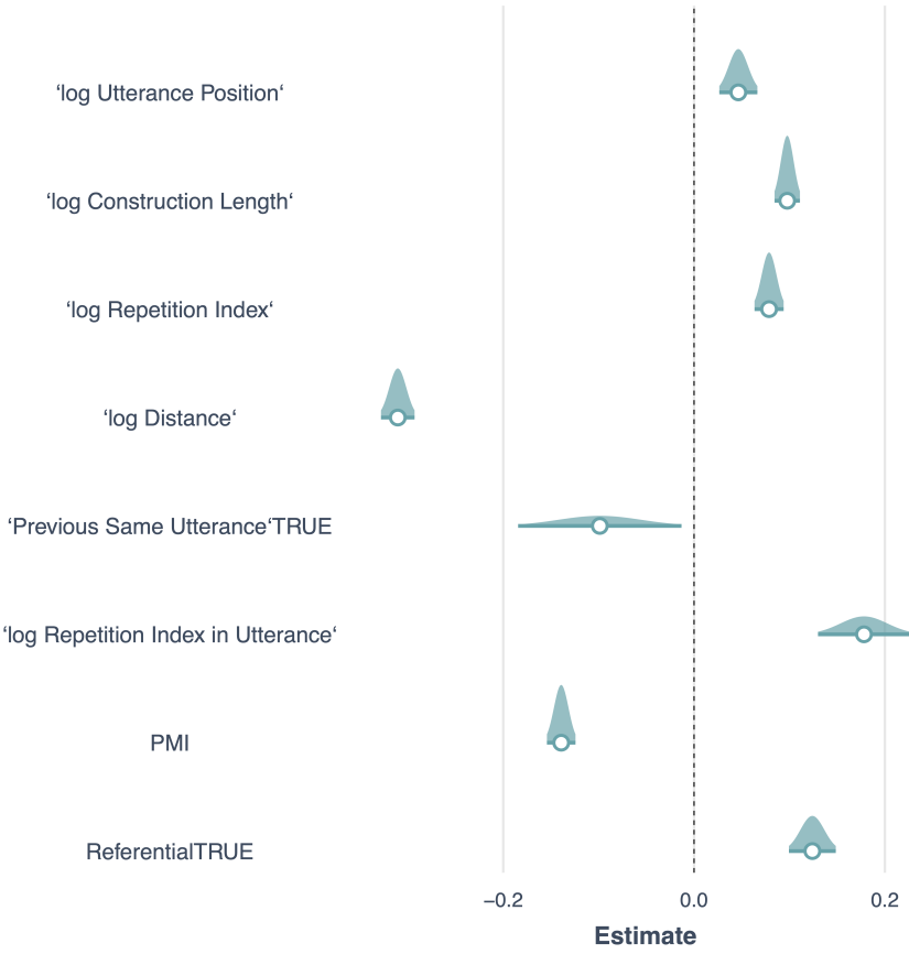
Figure B.4: Significant predictors of facilitating effect. Mixed effects linear regression, continuous predictors are mean-centred and scaled by 2 standard deviations.
