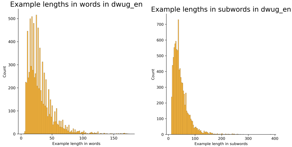
Figure A.4: Length distribution of usage examples in the English DWUGs.
