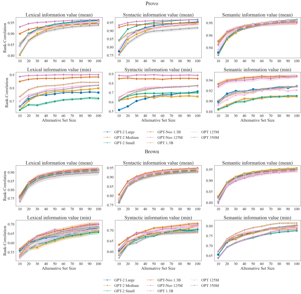
Figure C.9: Intrinsic evaluation on reading times corpora.
