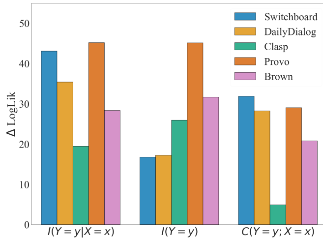
Figure 11.2: Explanatory power of information value and its derived measures, as defined in Section 11.6.1.
