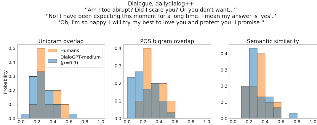
Figure 10.10: An example of well calibrated cross-variability in open-domain dialogue. D_{W_1}(C_k(x), H_k(x)) , DialogGPT Medium with nucleus sampling.
