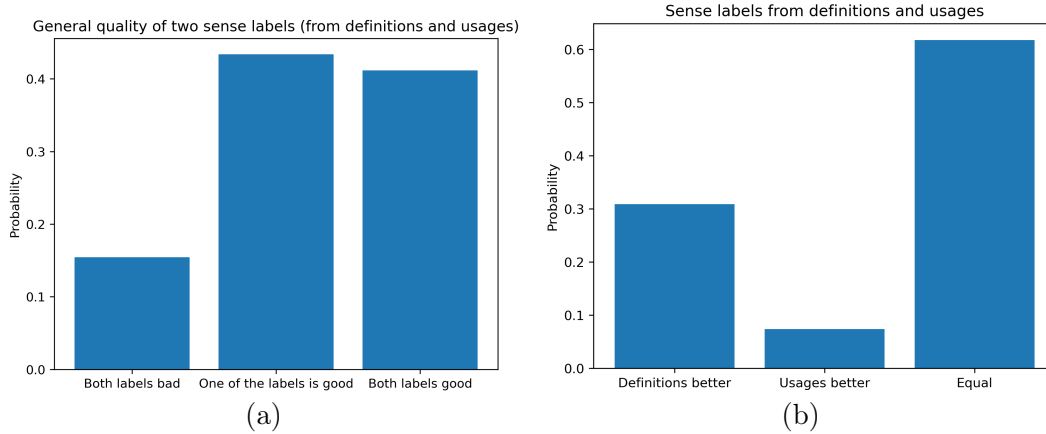
Figure 5.3: Human evaluation results: general quality of generated sense labels (a) and comparison between sense labels produced from definitions vs. usages.
