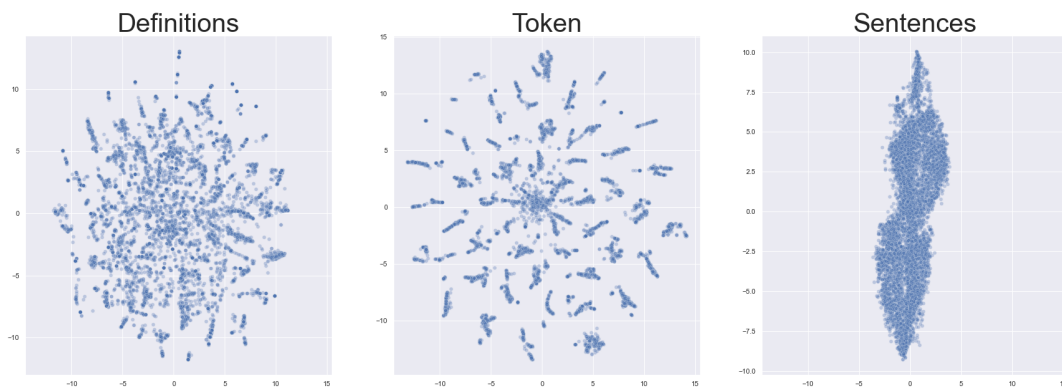
Figure A.6: T-SNE projection of each embedding space, RoBERTa-Large model.
