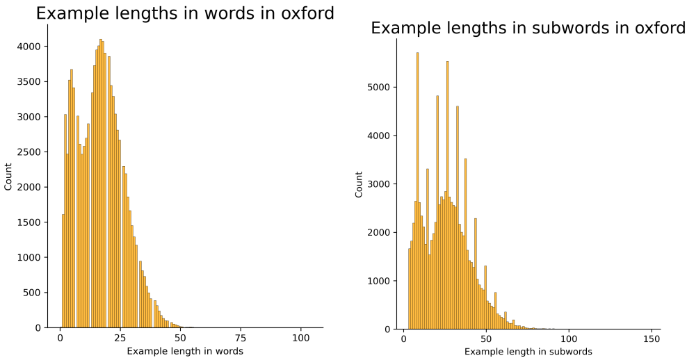
Figure A.2: Length distribution of usage examples in Oxford.
