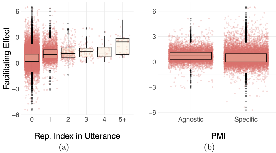
Figure 8.3: Facilitating effect against repetition index within the current utterance (a) and facilitating effect of interaction-agnostic constructions ( \text{PMI}(c, d) < 1 ) vs. interaction-specific constructions ( \text{PMI}(c, d) = \max_{c', d'} \text{PMI}(c', d') ) (b).
