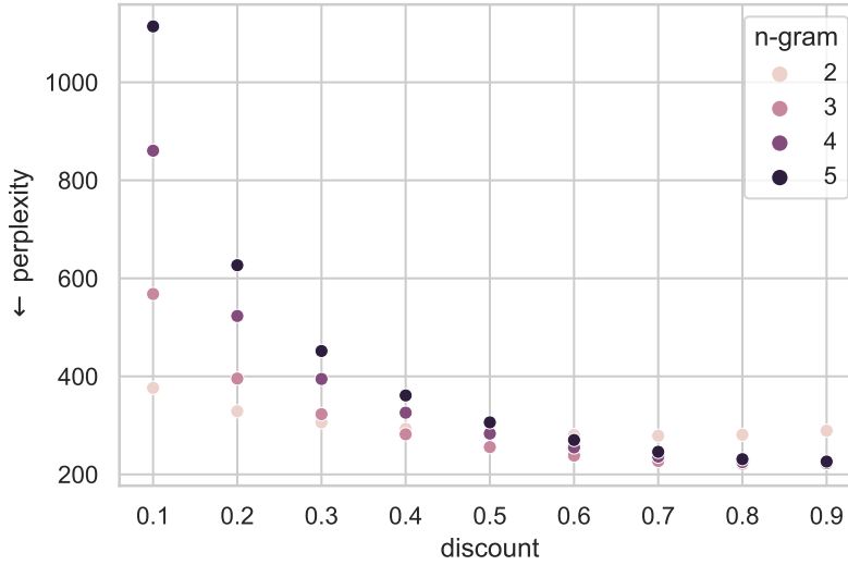
Figure B.1: Perplexity on Penn Treebank test set obtained by n -gram language models with Kneser-Ney smoothing and interpolation.
