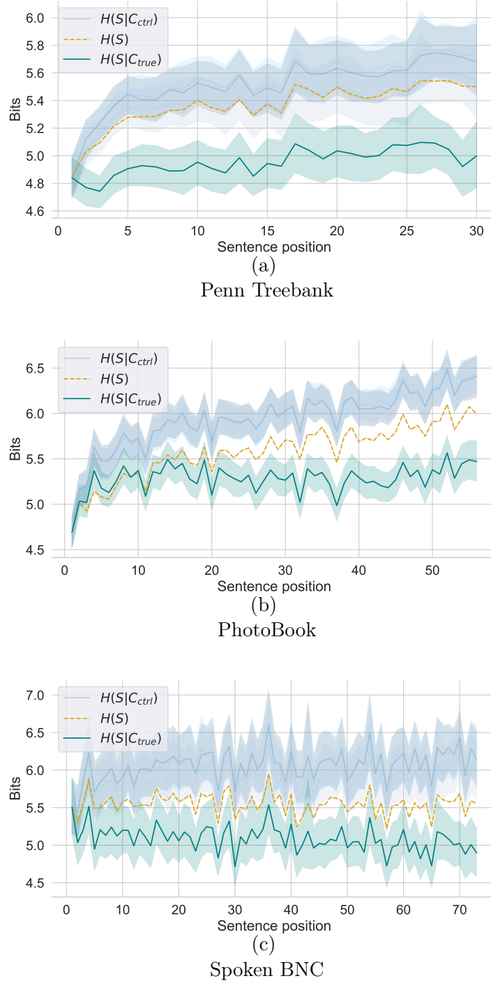
Figure 6.1: Contextualised surprisal estimates with true and random control contexts. Bootstrapped 95% confidence bands. We also show the mean H(S) values for reference (confidence bands will be visible in Figure 7.1).
