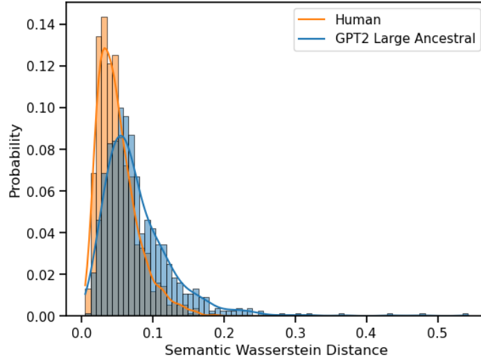
Figure 10.5: Distribution over Wasserstein distances D_{W_1}(C_{\text{sem}}(x), H_{\text{sem}}(x)) , in blue. Distances for a human control group, D_{W_1}(\hat{H}_{\text{sem}}(x), H_{\text{sem}}(x)) , in orange.
