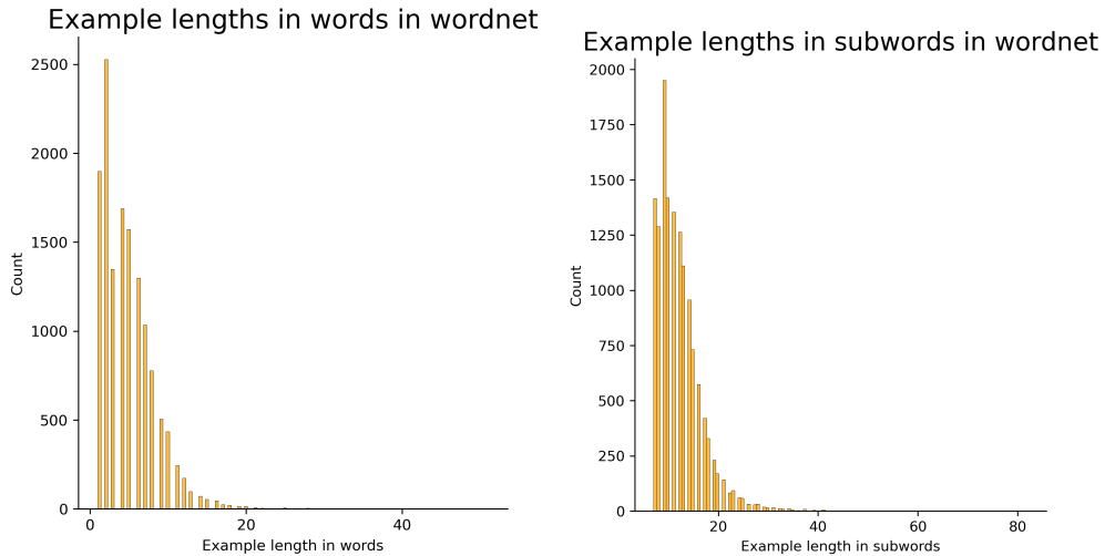
Figure A.1: Length distribution of usage examples in WordNet.
