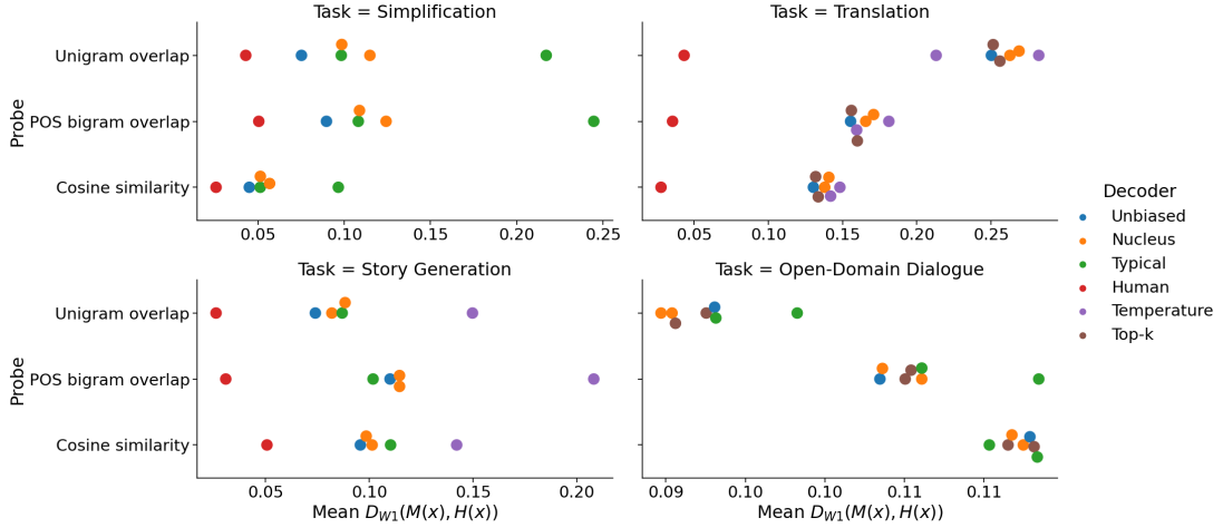
Figure C.3: Mean Wasserstein distances D_{W_1}(M(x), H(x)) for (tasks, probe, decoding algorithm) tuples. Base models for each task are described in Section 10.3. Tuples that share colour have different decoding parameters.
