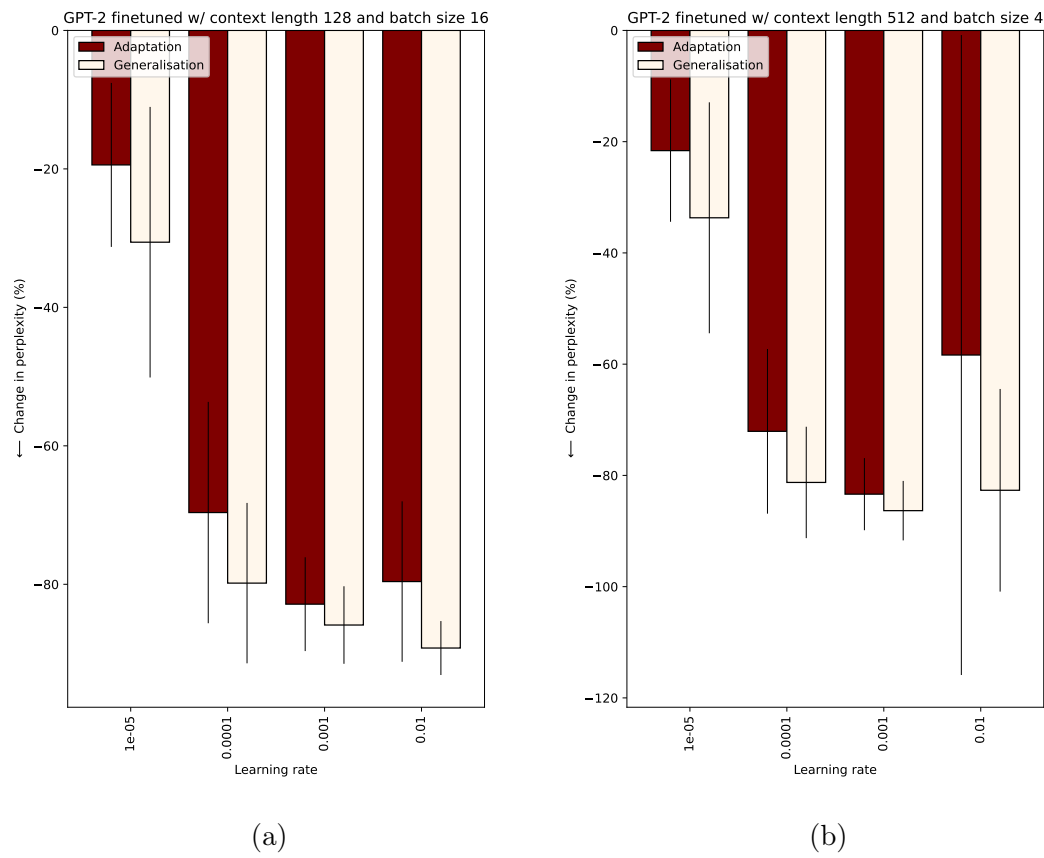
Figure B.3: The adaptation and generalisation performance (defined in Section B.6.2) with varying learning rate.
