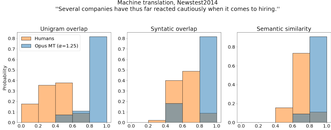
Figure 10.7: An example of variability underestimation in translation. Self-variability, D_{W_1}(M_k(x), H_k(x)) , OpusMT with temperature sampling.
