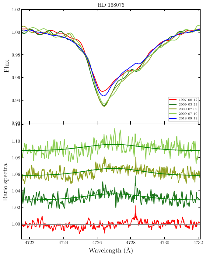
Fig. 2. Variation in \lambda 4727 DIB spectra towards HD 168076 used in this study. The EDIBLES spectrum is plotted in blue, and the earliest archival spectrum is in red; the intermediate observations are in green. The spectra are smoothed using a Gaussian convolution to minimize noise and better bring out the variations. The lower panel shows the ratio spectra and the fitted Gaussian model in each case. The top three ratio spectra (dividing the intermediate spectra by the EDIBLES spectrum) indicate significant variation, while the bottom ratio spectrum shows insignificant change when comparing the oldest archival to the EDIBLES observations.
