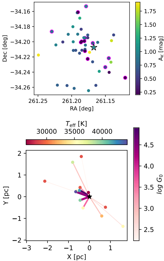
Figure 5. Top: extinction A_K for a sample of stars in Pis24, shown in colors. The position of XUE 1 in this diagram is indicated with a star. The O stars from the bottom panel are indicated with magenta borders. Bottom: radiation field toward XUE 1. The lines show the 2D distance from the massive stars to XUE 1 (indicated with the black star), and the colors of the circles show their temperature. The FUV radiation felt by XUE 1 from each massive star is shown by the color and width of the lines.
