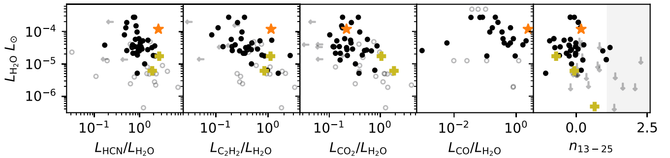
Figure 4. Comparison between the gas line luminosities and spectral index n_{13-25} of XUE 1 and the Spitzer sample studied by Banzatti et al. (2020) and the CO emission from Banzatti et al. (2022) (black circles). The y-axis shows the 17\ \mu\text{m} \text{H}_2\text{O} luminosity. From left to right the x-axis shows the ratio of HCN, \text{C}_2\text{H}_2 , \text{CO}_2 , and CO to \text{H}_2\text{O} luminosities. The x-axis of the rightmost panel shows the spectral index n_{13-25} , where the shaded region shows the location of disks with large gaps and/or cavities. The measurements for the JWST spectrum of XUE 1 are shown with the orange stars. The upper limits from Banzatti et al. (2020) and Banzatti et al. (2022) are indicated with gray arrows, and the open circles show the sources with upper limits in both the numerator and denominator. The yellow plus signs show the location of the MIRI spectra published to date: GW Lup (Grant et al. 2023), EX Lup (Kóspál et al. 2023), and PDS 70 (Perotti et al. 2023).
