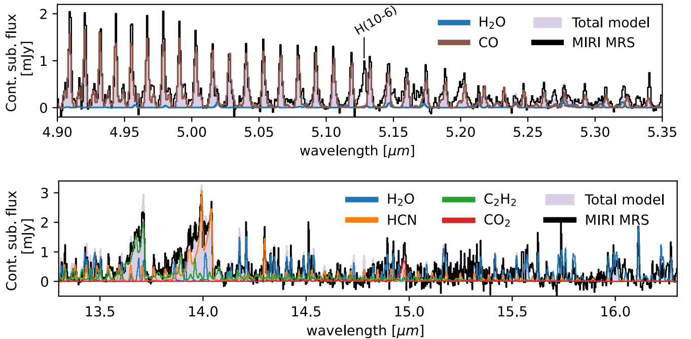
Figure 3. Continuum-subtracted MIRI spectrum of XUE 1 (black) with the best-fit slab models. Molecules are shown with colors, and the purple shaded area shows the total model spectrum. Top: region between 4.9 and 5.35 \mu\text{m} including CO (brown) and H 2 O (blue). Bottom: region between 13 and 16 \mu\text{m} including H 2 O (blue), C 2 H 2 (green), HCN (orange), and 12 CO 2 (red).
