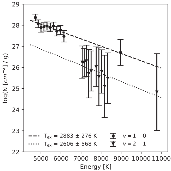
Figure 2. Rotation diagrams for the \nu = 1-0 (circles), \nu = 2-1 (triangles) bands. The dashed and dotted lines show linear fits to each vibrational level.
