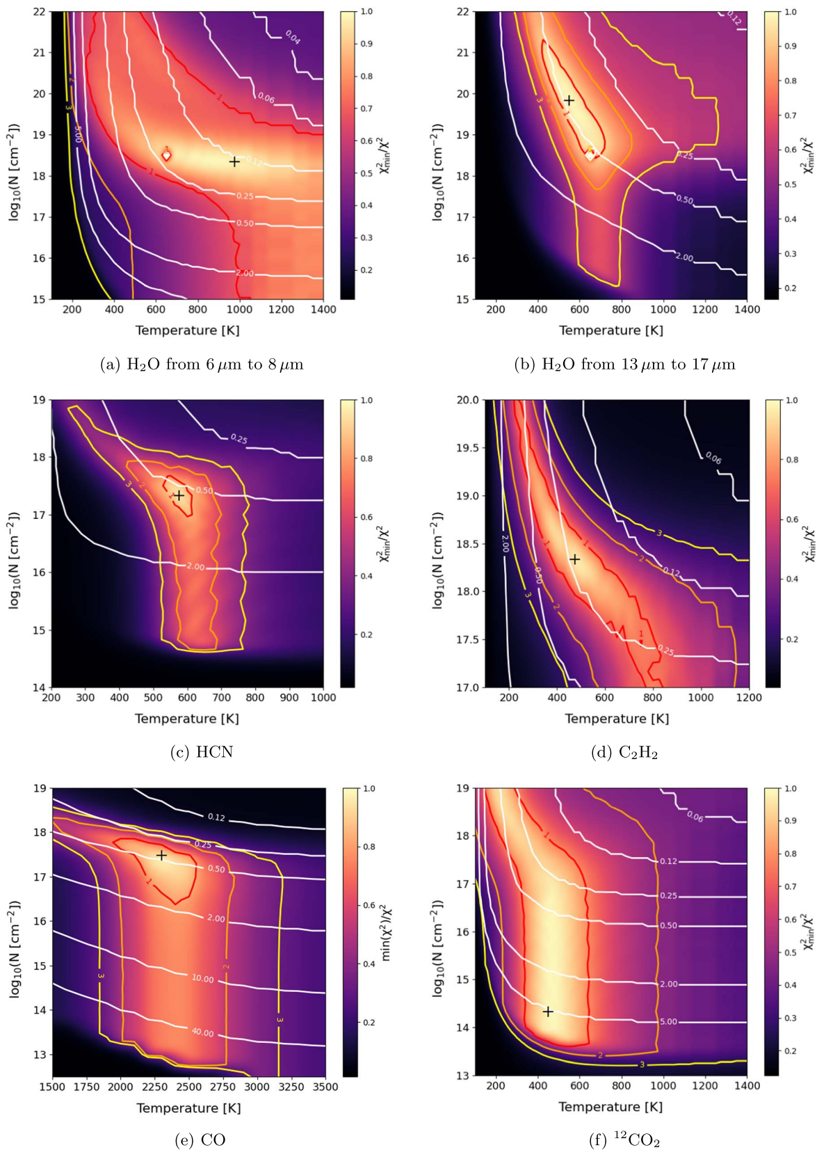
Figure 7. Reduced \chi^2 maps resulting from the fitting of LTE slab models to the MIRI MRS spectrum. The colors indicate the \chi_{\min}^2/\chi^2 value, with 1 being the best-fit model. The white contours show the emitting radius in au, and the red, orange, and yellow contours show the 1\sigma , 2\sigma , and 3\sigma confidence intervals. The location of the best-fit models in the parameter space is shown by a black plus sign.
