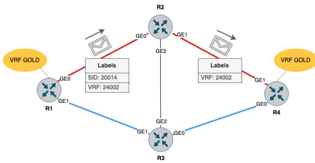
Fig. 2: Path chosen for FlexAlgo 128
