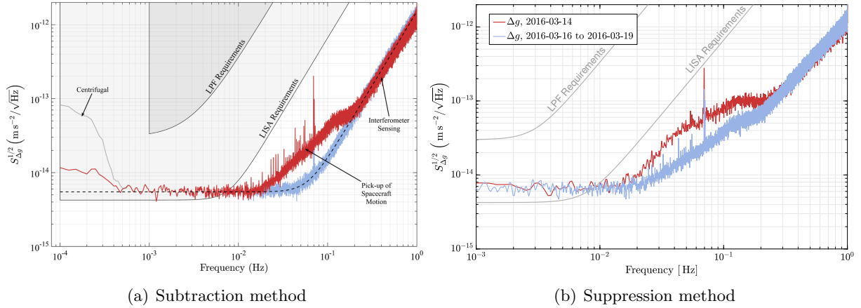
Figure 1. (a): Result taken from [1], showing that the bulge at 200-20 mHz can be subtracted. (b) In this figure, no subtraction was performed. Instead the reduction was achieved by a realignment of the test masses prior to the second noise run. 1
