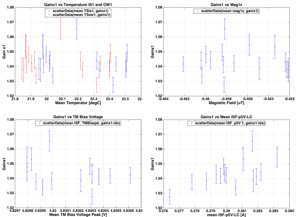
Figure 4. Gain trend for TM1 displacements with respect to the following parameters: temperature of the inertial sensors (left-hand side, top, blue), temperature of the optical window (left-hand side, top, red), TM bias voltage (left-hand side, bottom), magnetic field (right-hand side, top) and +5 V digital line consumption current in GRS (right-hand side, bottom).
