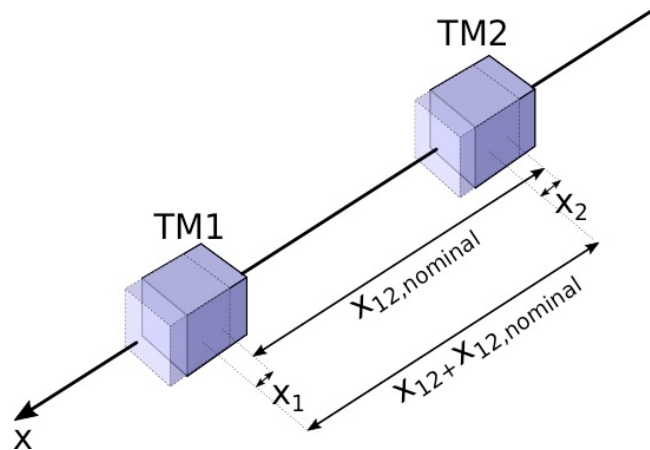
Figure 2. Illustration of test mass displacements and labelling the coordinates along the main measurement axis, x.
