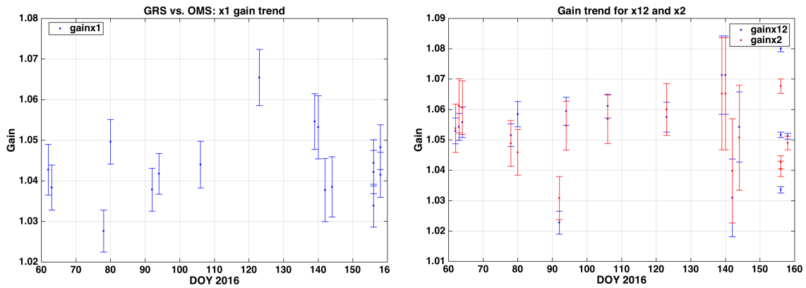
Figure 3. Gain trend resulted from the linear fit of GRS data to OMS data for TM1 (left-hand side), TM2 (right-hand side, red) and the differential displacement (right-hand side, blue).
