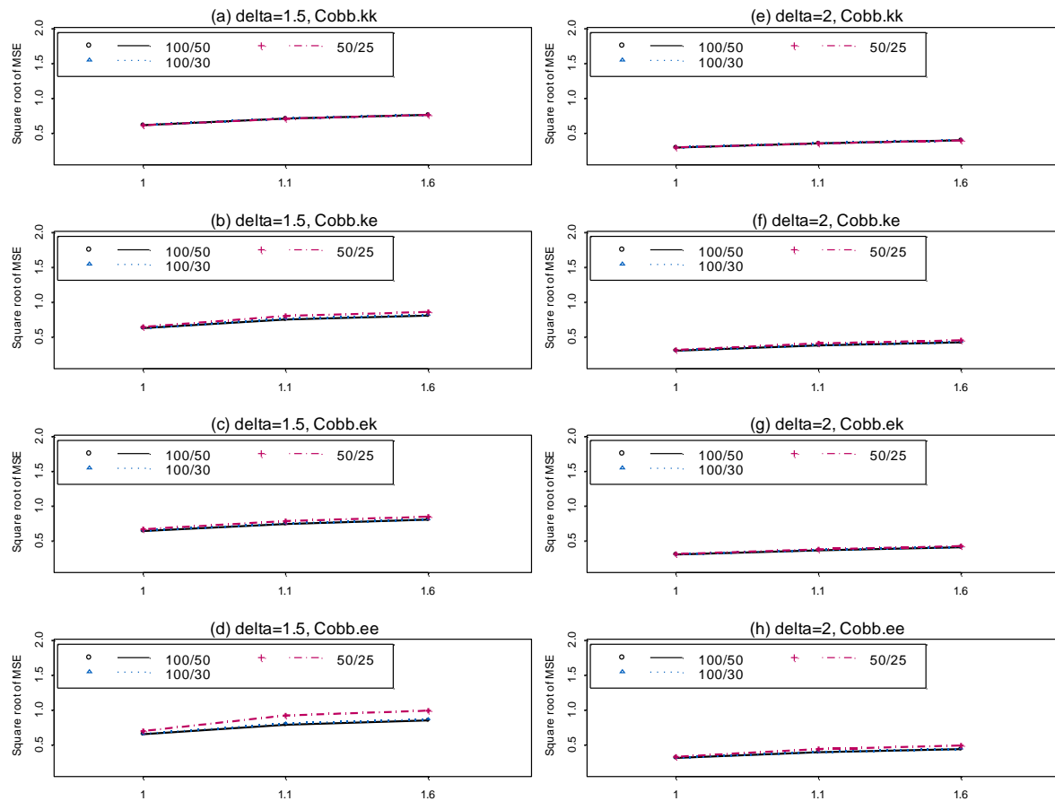
Figure 5.5 The effect of sample size and change-point position to the Cobb's estimation method for bivariate series.
