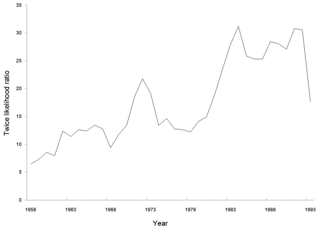
Figure 6.2: Twice log-likelihood ratio for a given change-point for the six rivers from the Northern Québec Labrador region..
